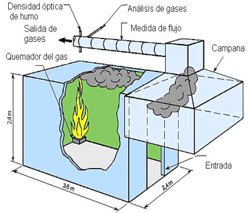
Fig. 2a-b. CEN/TS 45545-2:2006 Anexo B (fuente: SP Technical Research Institute of Sweden).
