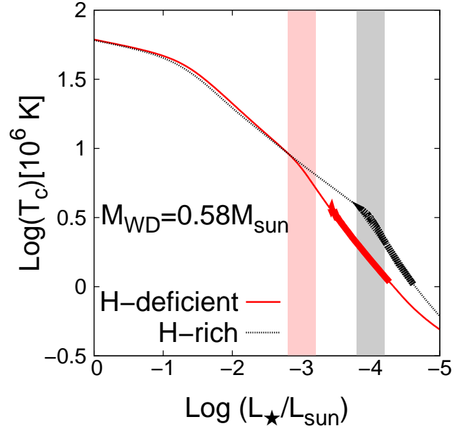
Figure 7. Central temperature in terms of the star luminosity for our 0.58 M_{\odot} hydrogen-deficient white dwarf model (solid red line), together with a 0.58 M_{\odot} hydrogen-rich model from Camisassa et al. (2016) (dotted black line). Thick segments indicate the core crystallization phase. Shaded areas indicate the occurrence of convective coupling.
