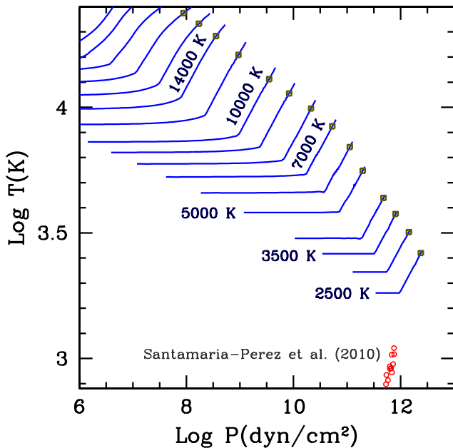
Figure 1. Temperature and pressure stratifications at 10^{-6} < \tau_{\text{Ross}} \leq 100 for helium atmospheres with \log g = 8 and various effective temperatures (some of them indicated on the plot). Squares display the optical depth \tau_{\text{Ross}} = 25.1189 where the atmospheres are attached to interior models. Circles show the melting data on helium reported by Santamaria-Pérez et al. (2010).
