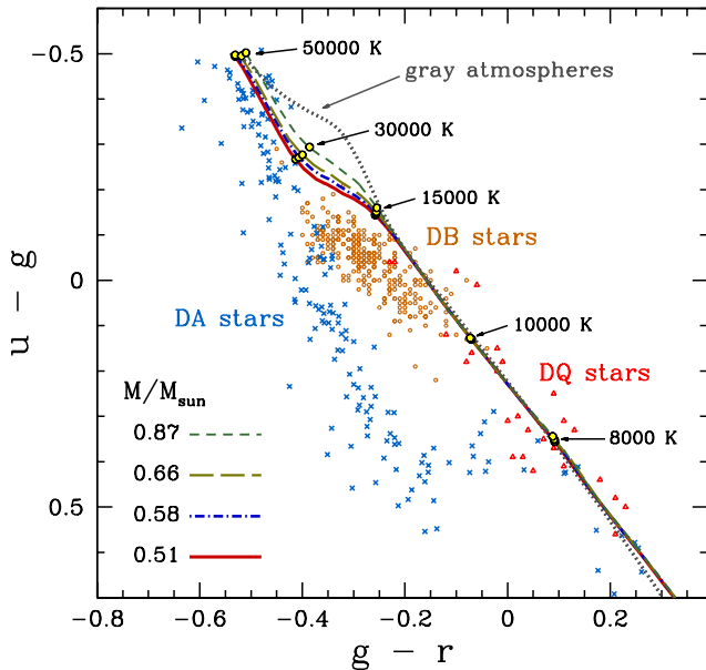
Figure 13. (u-g) versus (g-r) color-color diagram in the SDSS photometric system for the 0.51, 0.58, 0.66 and 0.87 M_{\odot} cooling tracks of hydrogen-deficient white dwarfs. The 0.87 M_{\odot} curve is labeled with effective temperatures. The dotted line displays the same evolutionary tracks calculated considering the gray approximation. Open circles are the DB white dwarfs studied by Koester & Kepler (2015), open triangles are the DQ white dwarfs studied by Harris et al. (2003) and Kleinman et al. (2004), and crosses are the DA white dwarfs studied by Holberg & Bergeron (2006).
