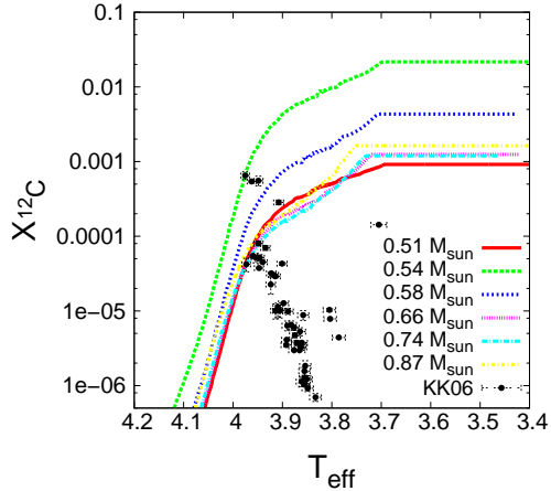
Figure 10. Surface mass fraction of ^{12}\text{C} in terms of the effective temperature for all our white dwarf sequences. Filled circles are the DQ white dwarfs studied by Koester & Knist (2006).
