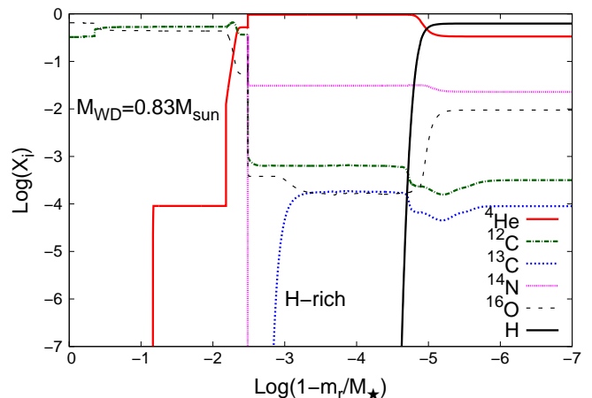
Figure 5. Upper panel: initial chemical profiles for our 0.87 M_{\odot} hydrogen-deficient white dwarf model in terms of the outer mass fraction. Bottom panel: initial chemical profiles for a 0.83 M_{\odot} hydrogen-rich white dwarf model (Camisassa et al. 2016)
