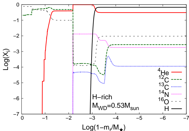
Figure 4. Upper panel: initial chemical profiles for our 0.51 M_{\odot} hydrogen-deficient white dwarf model in terms of the outer mass fraction. Bottom panel: initial chemical profiles for a 0.53 M_{\odot} hydrogen-rich white dwarf model (Camisassa et al. 2016)
