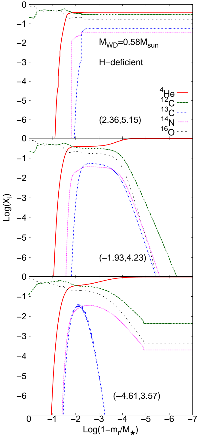
Figure 8. Abundance by mass of {}^4\text{He} , {}^{12}\text{C} , {}^{13}\text{C} , {}^{14}\text{N} and {}^{16}\text{O} as a function of the outer mass fraction, \log(1 - m_r/M_\star) , for our 0.58 M_\odot white dwarf model at three selected evolutionary stages. The logarithm of the luminosity (in solar units) and the logarithm of the effective temperature are indicated in brackets in each panel.
