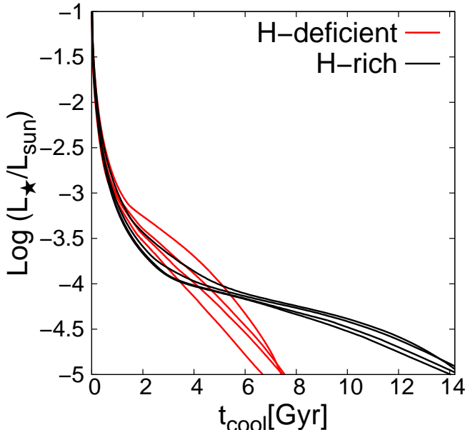
Figure 11. White dwarf evolutionary times. The red solid lines indicate four hydrogen-deficient white dwarf sequences calculated in this work. At t_{\text{cool}} = 6 Gyr and from bottom to top, the different lines display the 0.51 , 0.58 , 0.66 and 0.87 M_{\odot} model sequences, respectively. Black solid lines correspond to hydrogen-rich white dwarf tracks with similar masses from Camisassa et al. (2016).
