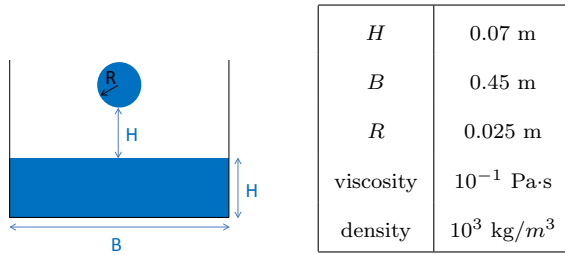
Fig. 24: Mixing of a viscous fluid. Initial geometry.
