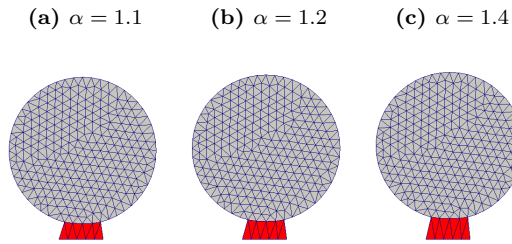
Fig. 23: Impact of a viscous fluid against a rigid wall. Snapshots at the contact instant for the three different values of the parameter \alpha .
