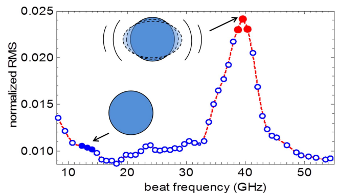
Figure 24. EAR spectroscopy used to probe the elastic vibrations of nanoparticles in a double nanohole. Two trapping lasers are used to produce a beating intensity, which drives the vibrations through electrostriction. Greater noise (normalized RMS variation) is seen at a vibrational resonance.
