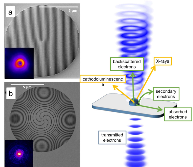
Figure 32. Scultured electrons, such as electron vortex beams, can interact with matter in new ways due to the non-trivial topology of the wavefront. Electron vortex beams are produced using nanofabricated diffraction holograms. Panels (a, b) reproduced with permission from [216]. Copyright 2014 IOP Publishing Ltd.
