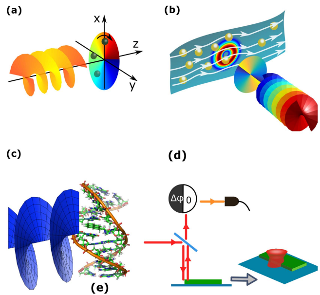
Figure 19. Applications of structured light to: (a) laser remote sensing, (b) vorticity in fluids, (c) optical activity in chiral molecules and (e) thin film measurement.
