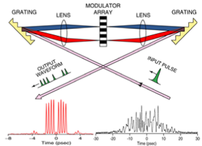
Figure 33. Femtosecond pulse shaper arrangement and representative ultrafast waveforms.
