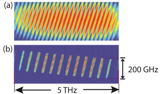
Figure 34. Dispersion of optical frequencies in 2D at the Fourier plane of a pulse shaper, without (a) and with (b) spectral shaping. Adapted with permission from [231]. Copyright 2008 the Optical Society.
