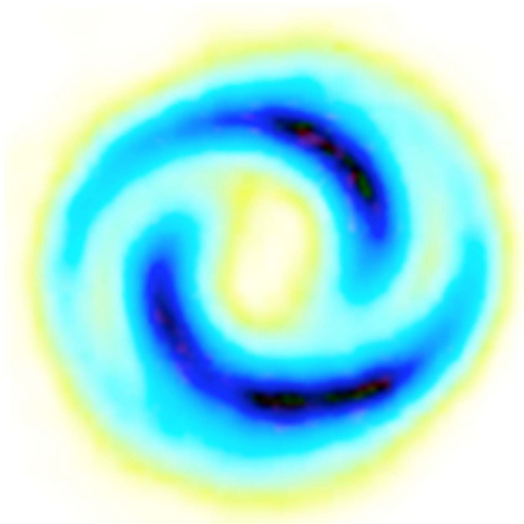
Figure 17. The density profile of one spin state of a spinor BEC that has counter rotating azimuthal phase twists (counter rotating vortices) and a radial phase gradient. See [119].
