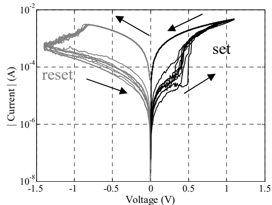
Fig.2: Resistive switching behavior during successive set and reset operations.
