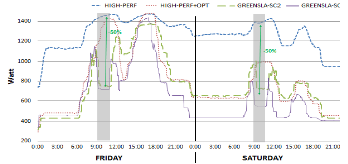
Fig. 6. Power consumption (Watt) of the tested scenarios
