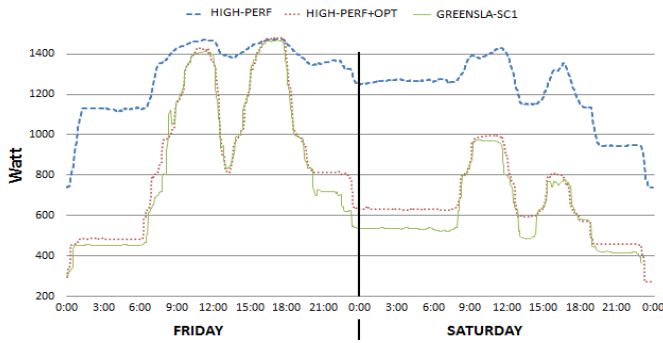
Fig. 4. Power consumption (Watt) of the tested scenario
