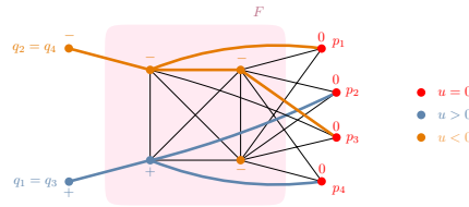
Fig. 2. Sign pattern in a non–planar network
