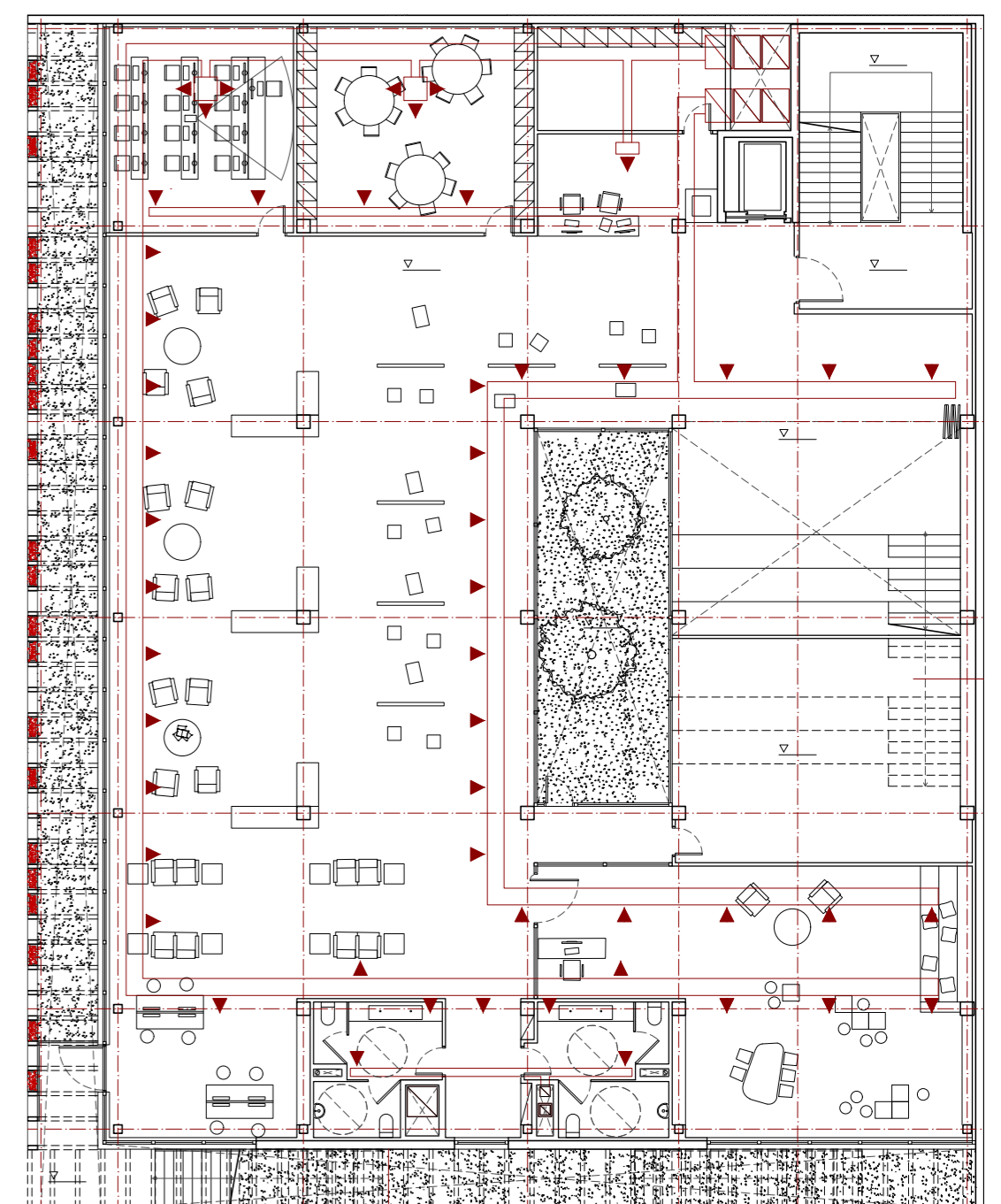
PB+1 1:200
