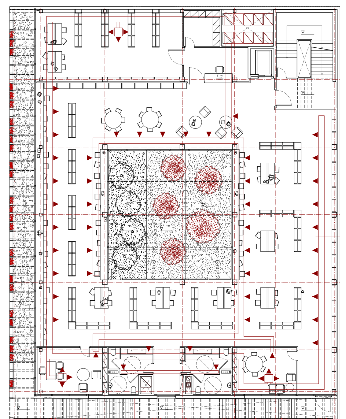
PB+3 1:200
