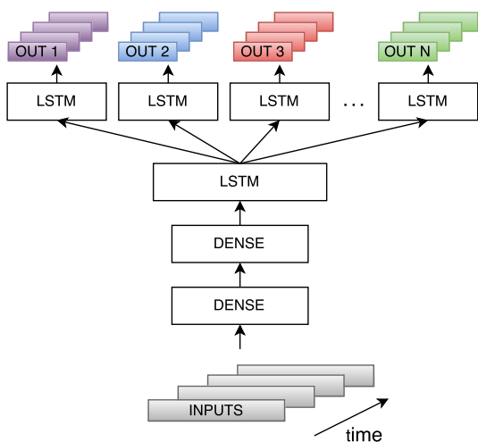
Figure 1: Proposed architecture using regular feed forward (dense) layers and recurrent LSTM layers. There are N outputs belonging to N different speakers.
