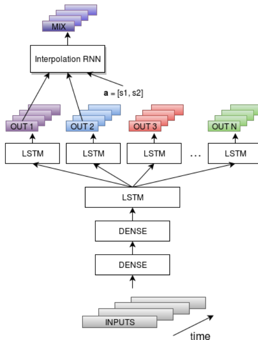
Figure 2: Example of \alpha -interpolated multi-output model with M = 2 .
