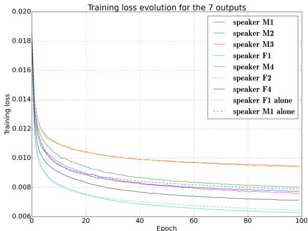
Figure 3: Training loss evolution comparison. Speakers F1 and M1 decrease the learning cost when trained with other speakers altogether.
