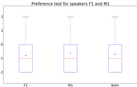
Figure 4: Box plot of preference test scores. Scores range from -2 (multiple output model is preferred) to 2 (single output trained model is preferred). Both is the summary of all the answers, joining both speaker results. Red lines mark the median and blue dots the mean.
