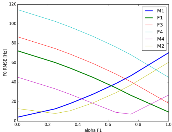
Figure 6: F0 RMSE when varying \alpha values. The variation is made for speaker F1 and it is (1-\alpha) for M1. All others speakers remain 0. M = 6 .
