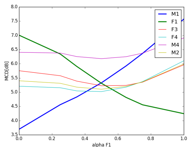
Figure 5: MCD when varying \alpha values. The variation is made for speaker F1 and it is (1 - \alpha) for M1. All others speakers remain 0. M = 6 .
