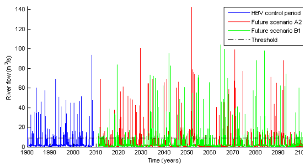
Fig. 9. Time series of the discharge values in the Anoia sub-basin. The HBV simulations for the control (1980–2008) period (blue) is plotted. The future (2011–2100) discharge series computed with the HBV model for the A2 (red) and B1 (green) SRES scenarios are also presented. The dashed black line represents the threshold of 9 \text{ m}^3 \text{ s}^{-1} .
