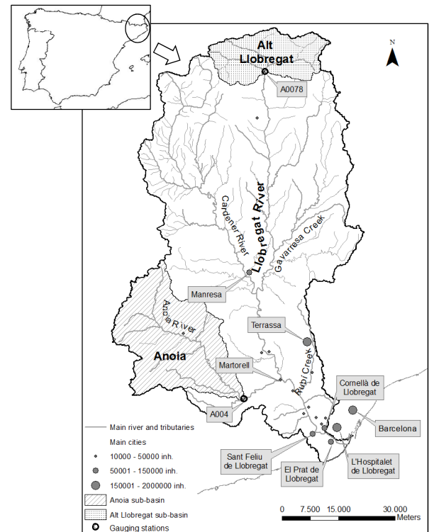
Fig. 1. Location of the Llobregat River basin.
