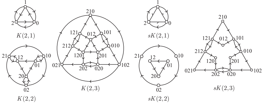
Figure 1: Some examples of Kautz and subKautz digraphs.
