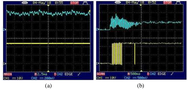
Figure 10. Voltage and current in the side motor (a) steady state, (b) start.
