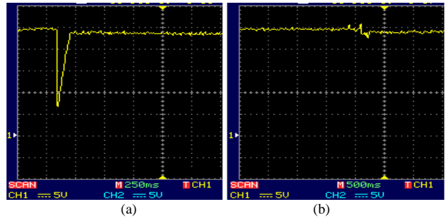
Figure 11. Power supply to the piston-boot (a) direct, (b) progressive start.
