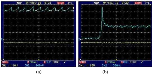
Figure 9. Voltage and current in the main motor (a) steady state, (b) start.
