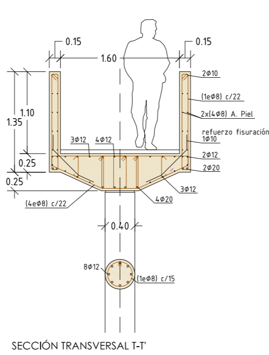
DETALLES RAMPA E:1/50
