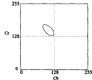
Fig. 3. Region bounding the skin-like colors on the C_bC_r color space.
