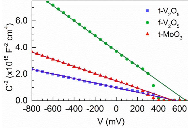
Figure 3: Experimental (dots) Mott-Schottky plots and respective linear fittings (lines) under dark and room temperature conditions for the different samples, as indicated. The AC perturbation was 10 mV at 1.0 kHz.
