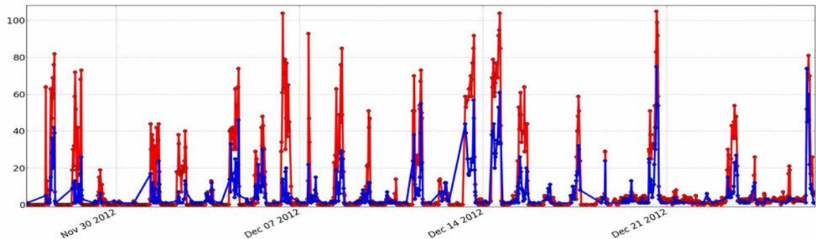
Fig 3. Fish counting trend of a time-series fragment, performed manually (red line) and automatically by the learnt classifier (blue line).
