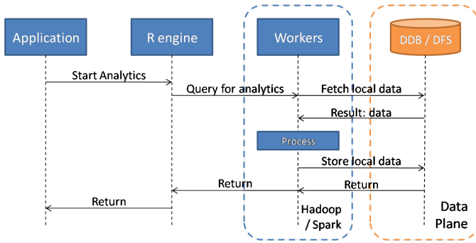
Fig. 2. Schema of distributed execution approach, with Distributed Databases or File Systems
