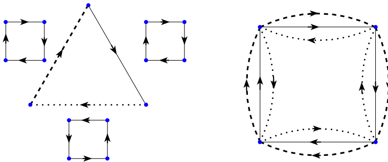
FIGURE 1. A function h : E(C_3^+) \rightarrow \Gamma and the multidigraph M_h .
