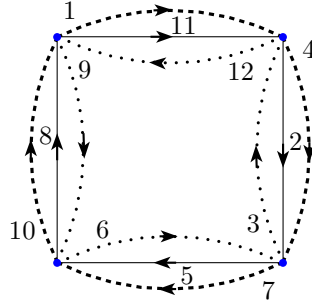
FIGURE 2. A rainbow eulerian circuit of M_h with color sequence (dash, line, dots).
