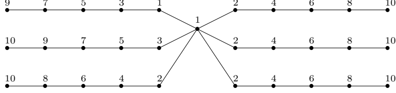
FIGURE 1. A proper distance 10-labeling of S_6^5 .
