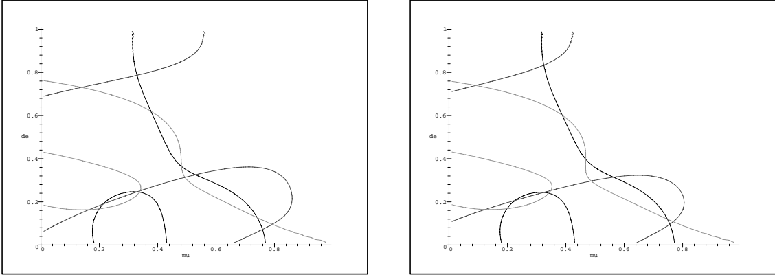
Figure 6: \lambda = 0.51 , \lambda = 0.52
