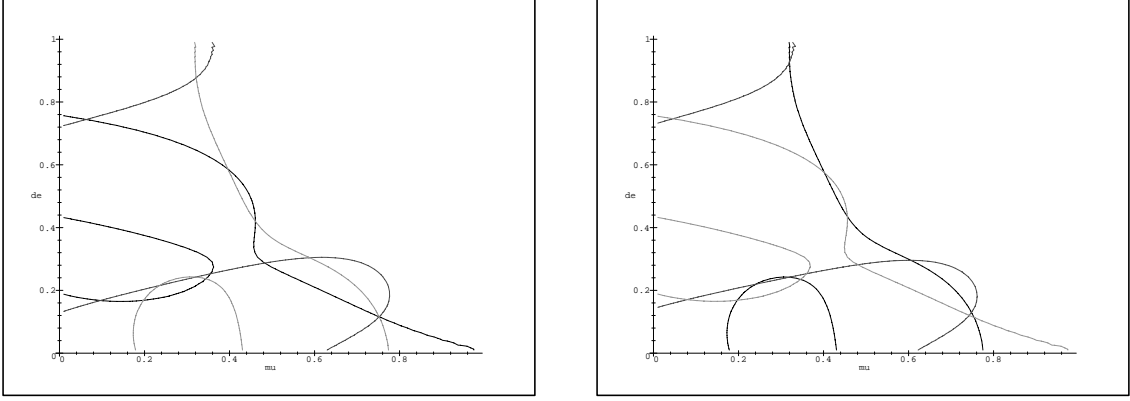
Figure 7: \lambda = 0.5267 , \lambda = 0.53
