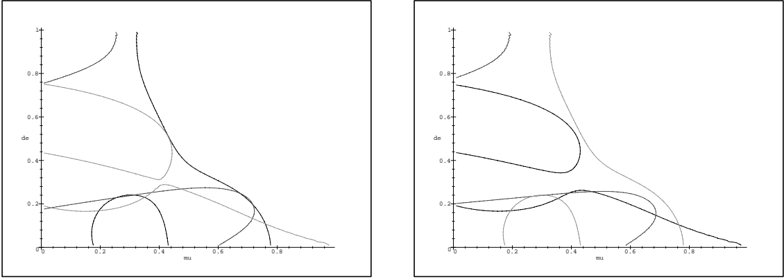
Figure 8: \lambda = 0.54 , \lambda = 0.55
