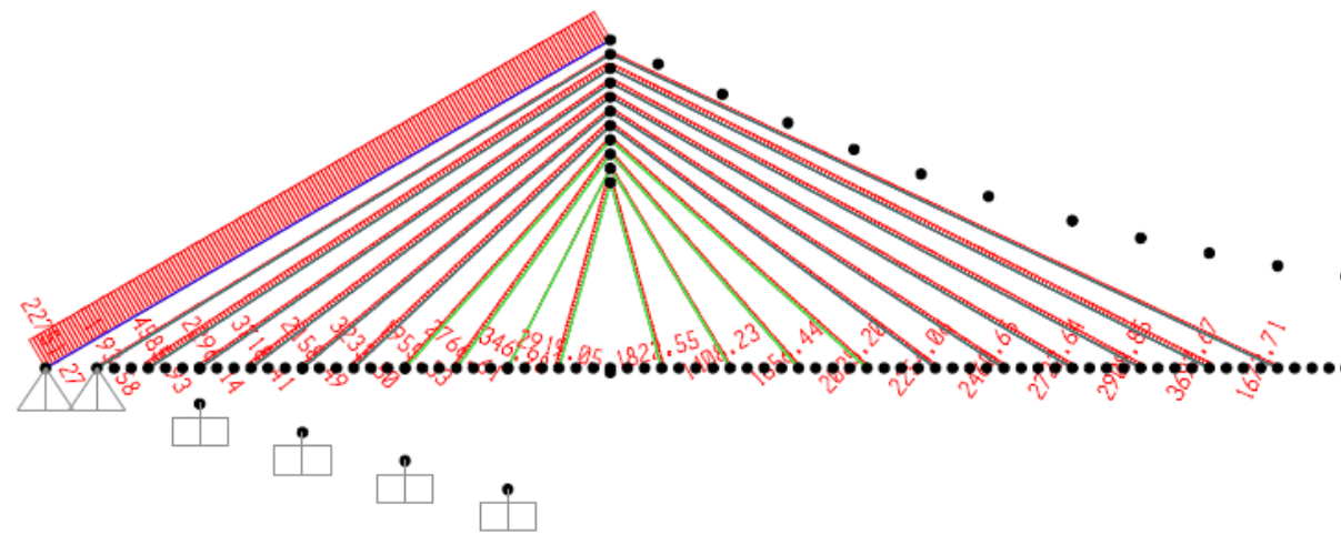
Image 12: Axial forces in phase 4
