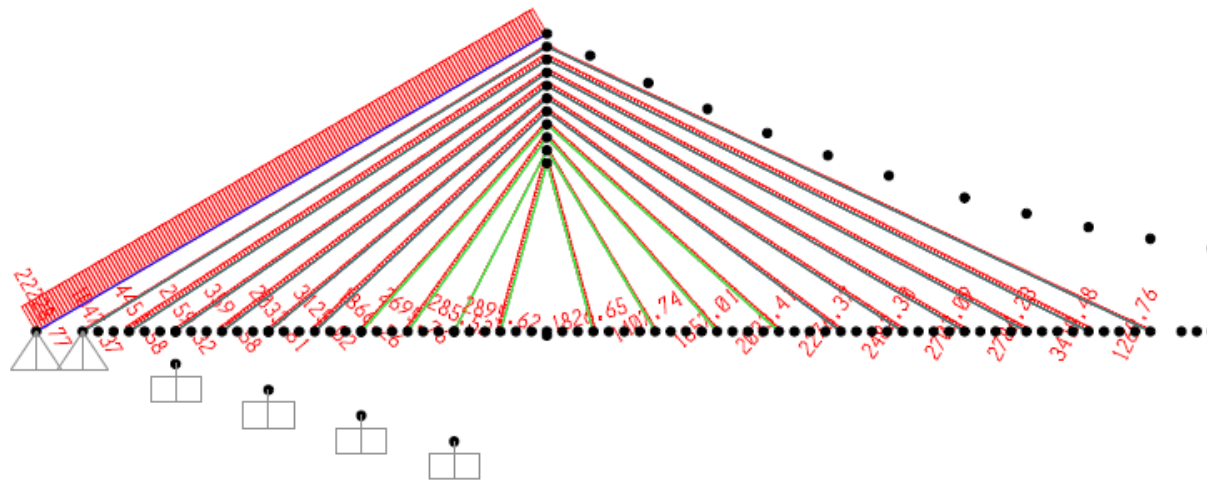
Image 11: Axial forces in phase 3
