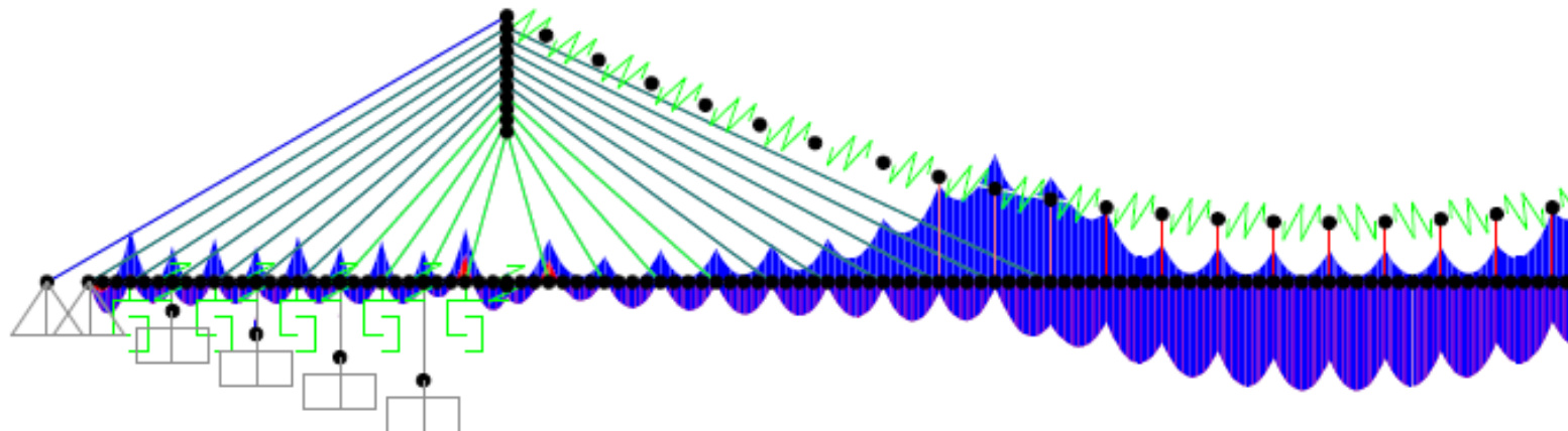
Image 15: Moment diagram in Comb 71
