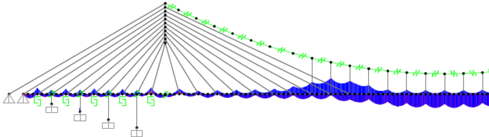
Image 8: Moment diagram in Comb 31
