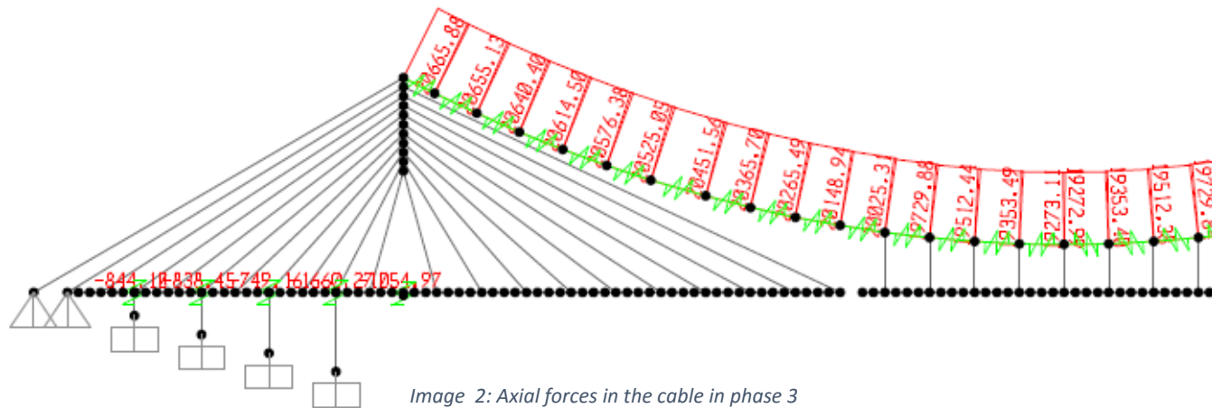
Image 2: Axial forces in the cable in phase 3
