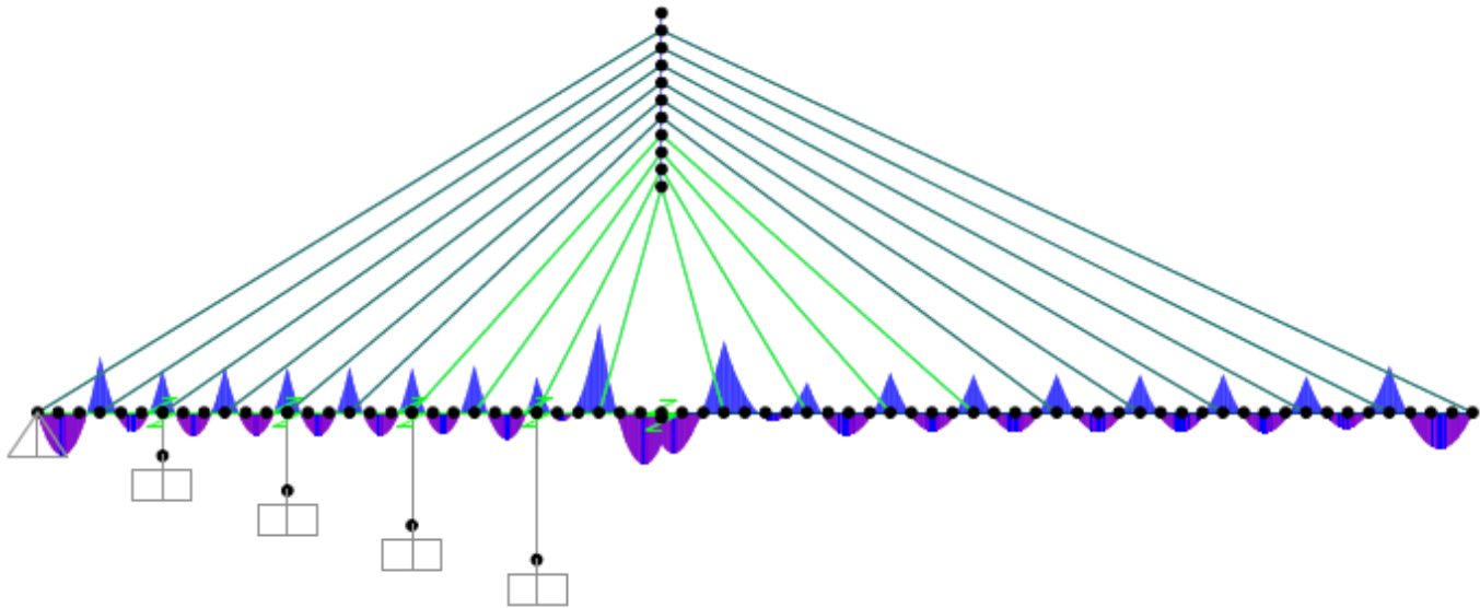
Image 5: Moment diagram in phase 1
