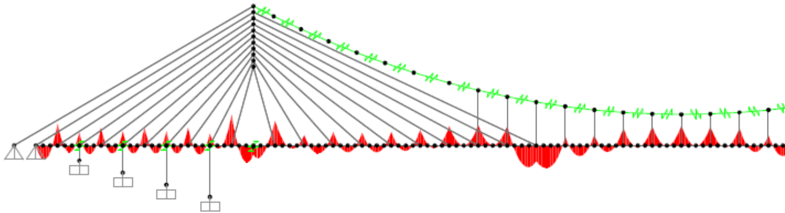
Image 7: Moment diagram in phase 4
