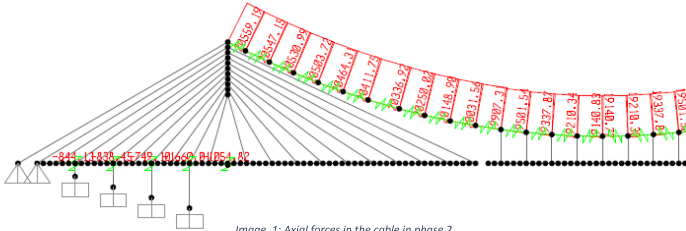
Image 1: Axial forces in the cable in phase 2
