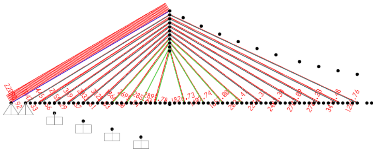
Image 10: Axial forces in phase 2
