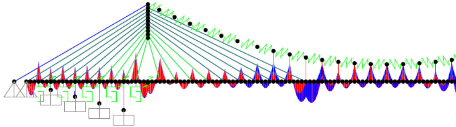
Image 14: Moment diagram in Comb 41
