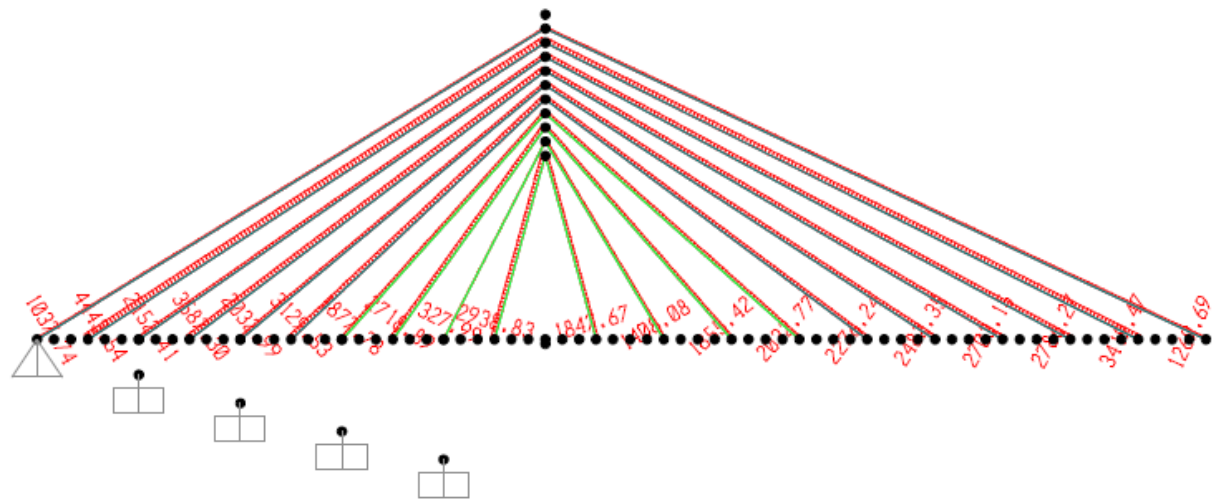
Image 9: Axial forces in phase 1
