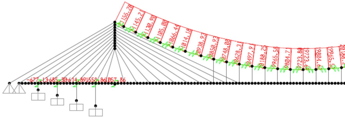
Image 3: Axial forces in the cable in phase 4
