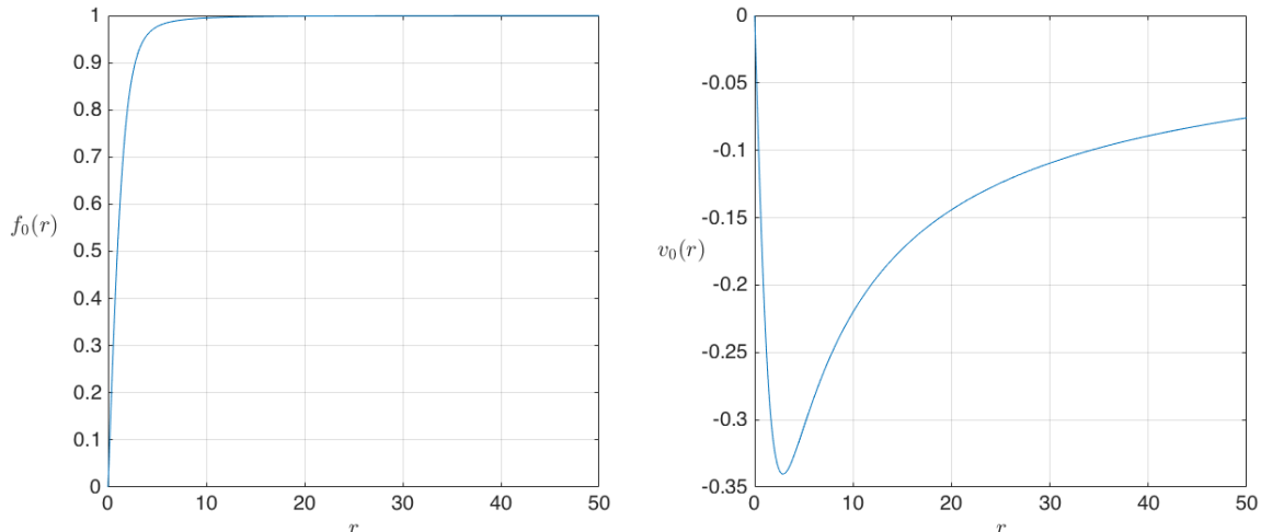
FIGURE 3. Leading order terms: solutions of (18)-(19).
