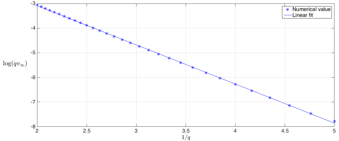
FIGURE 2. Value of \log(qv_\infty) as a function of 1/q , with q \in [0.2, 0.5] for the system (14)-(15).
