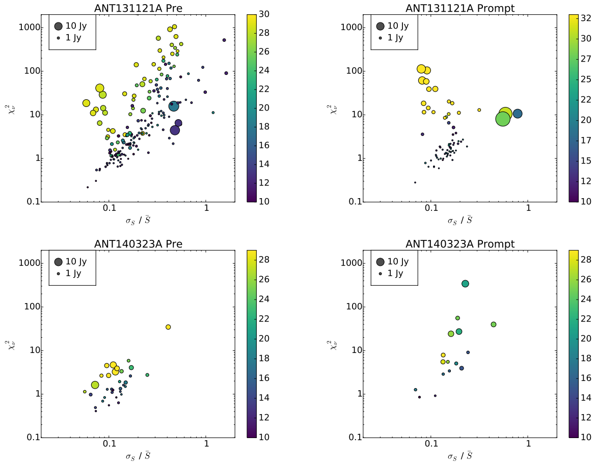
Figure 2. Reduced chi-squared, \chi_r^2 , for the hypothesis that sources do not vary over the \sim 30 snapshots, plotted against fractional modulation (standard deviation, \sigma_s , divided by the mean, \bar{S} , flux density for the same sources). Sources are color-coded according to the number of snapshots in which they were detected. Data are plotted for pre-trigger (left) and prompt (right) datasets, for ANT 131121A (top) and ANT 140323A (bottom). Only sources detected in \geq 10 of the snapshot images for each dataset are shown. Circle sizes scale with \bar{S} .
