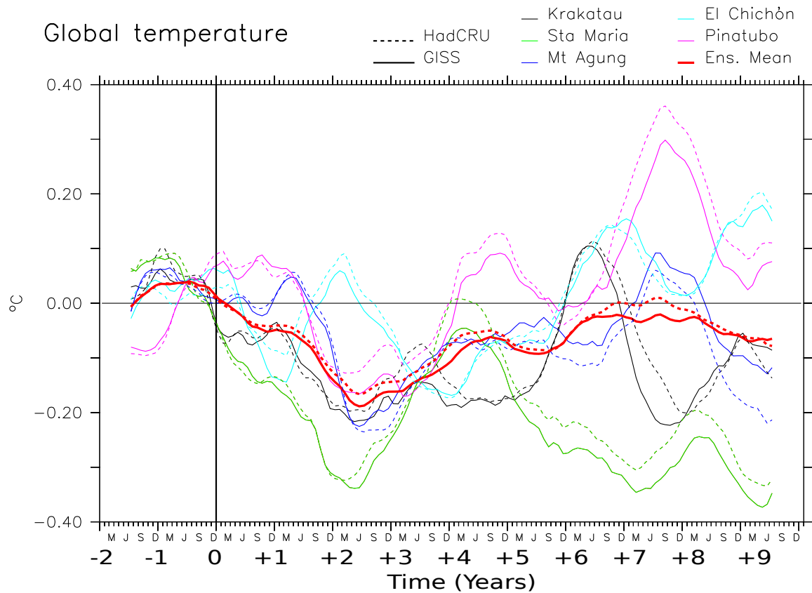
Figure 4: Anomalous global atmospheric temperature at the Earth's surface (in °C) in response to five major volcanic eruptions over the instrumental era (Krakatau in 1883, Santa María in 1902, Agung in 1963, El Chichón in 1982 and Pinatubo in 1991) from GISS (continuous lines, Hansen et al. 2010) and HadCRU (dashed lines, Morice et al. 2012) datasets. The anomalies refer to the average of the three-year preceding each eruption. The vertical line stands for the year when the onset of the eruptions occurs. The unit of the x-axis is year.
