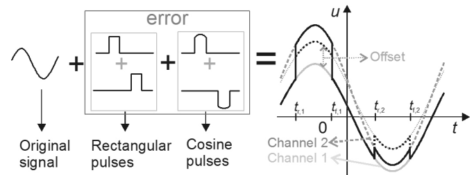
Modelling of errors of MRADC system: Sketch of COS model formation based on time domain pulses
