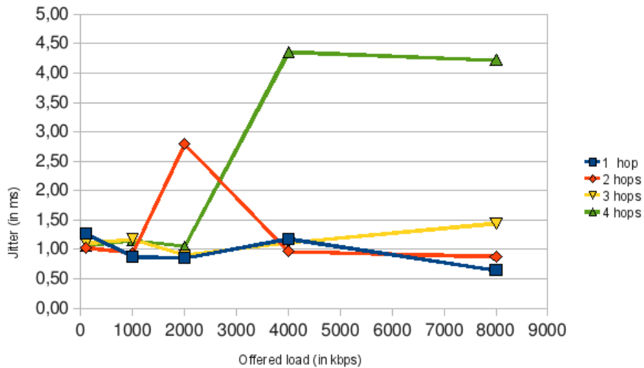
Figure 4.14: OLSR evaluation of Jitter
