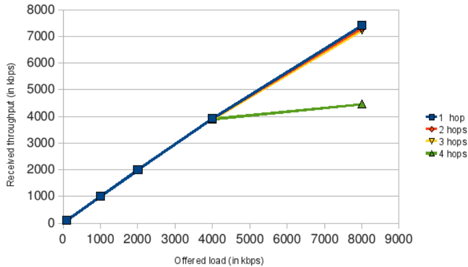
Figure 4.8: OLSR evaluation of UDP bandwidth
