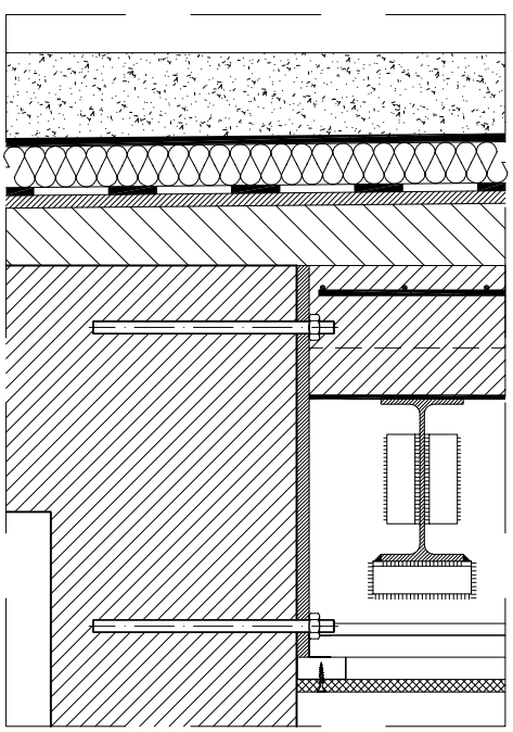
Detall B (e: 1/5)
