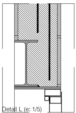
Detall L (e: 1/5)
