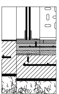
Detall Q (e: 1/5)
