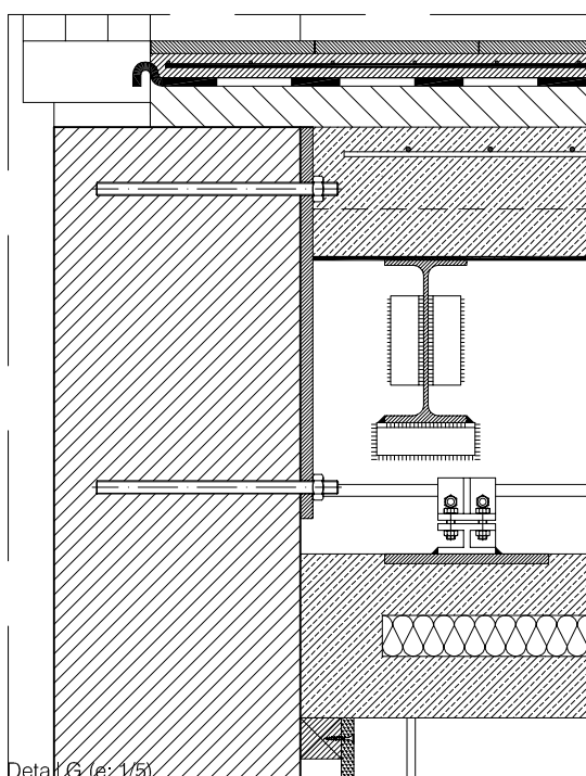
Detall G (e: 1/5)
