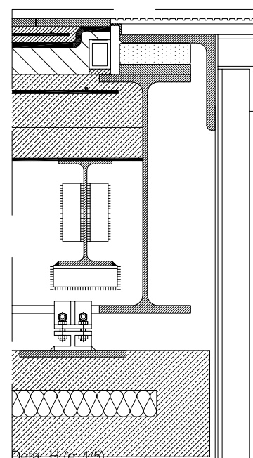
Detall H (e: 1/5)
