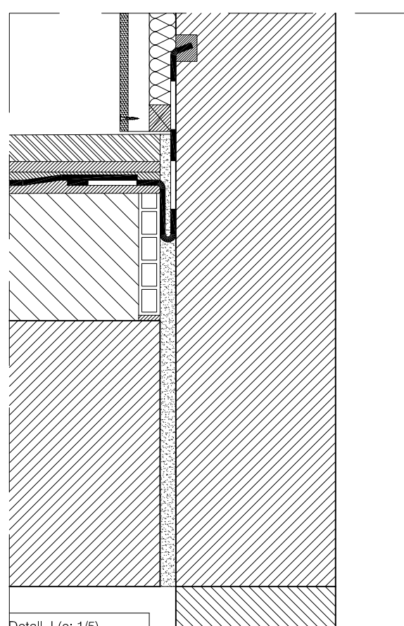
Detall J (e: 1/5)
