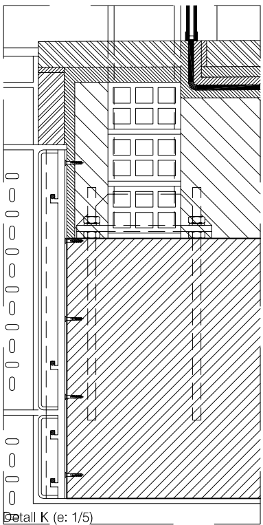
Detall K (e: 1/5)
