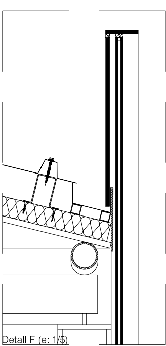
Detall F (e: 1/5)
