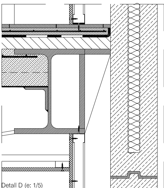
Detall D (e: 1/5)
