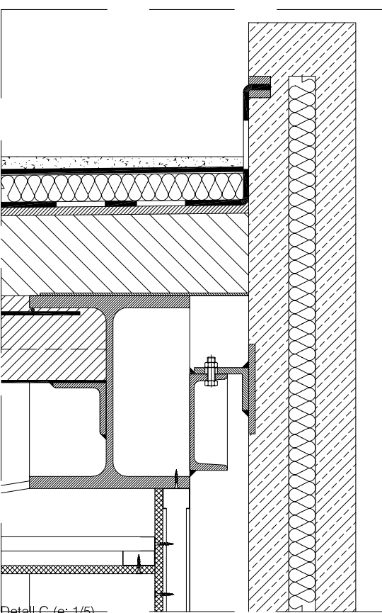
Detall C (e: 1/5)
