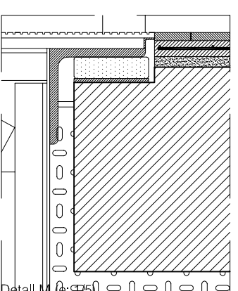
Detall M (e: 1/5)
