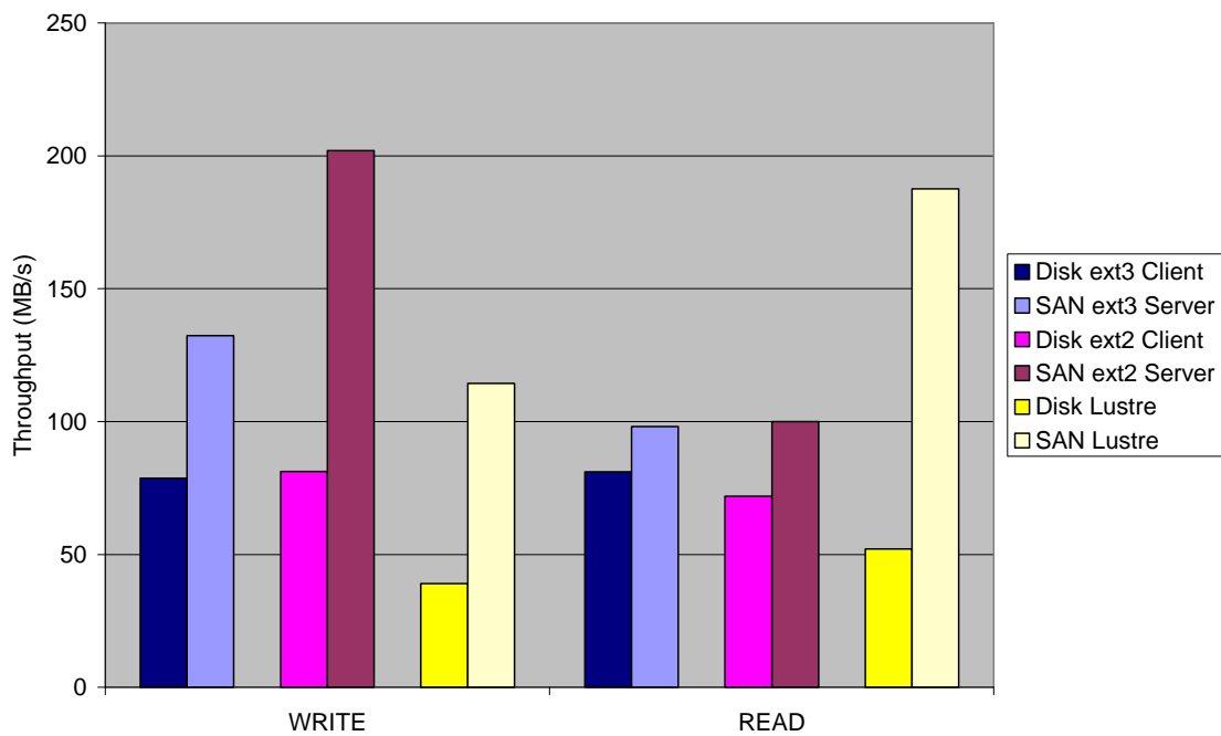
Figure 39 - Local throughput
