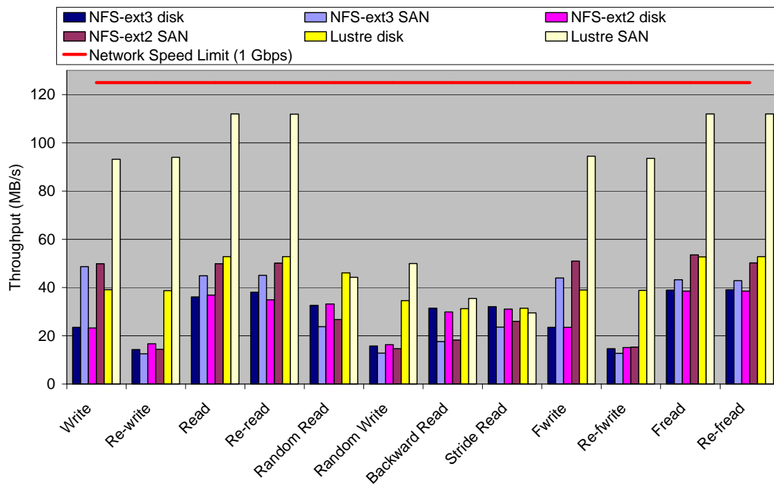
Figure 40 - Remote throughput
