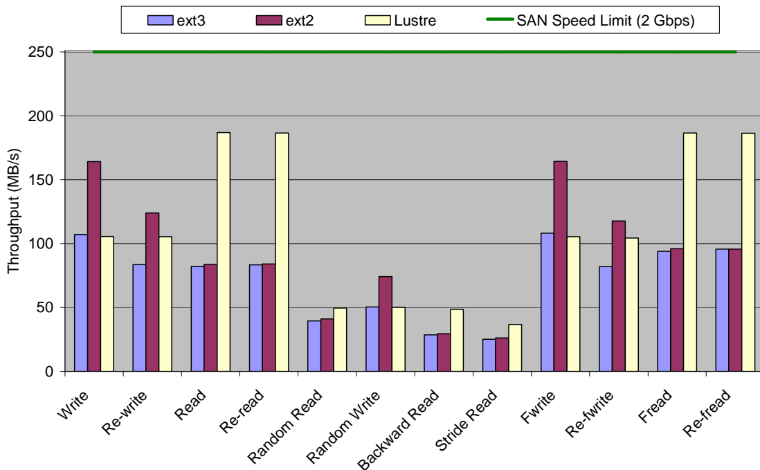
Figure 12 - Local throughput
