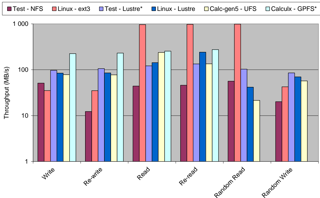
Figure 21 - Computing system throughput tests with a 5 GB file
