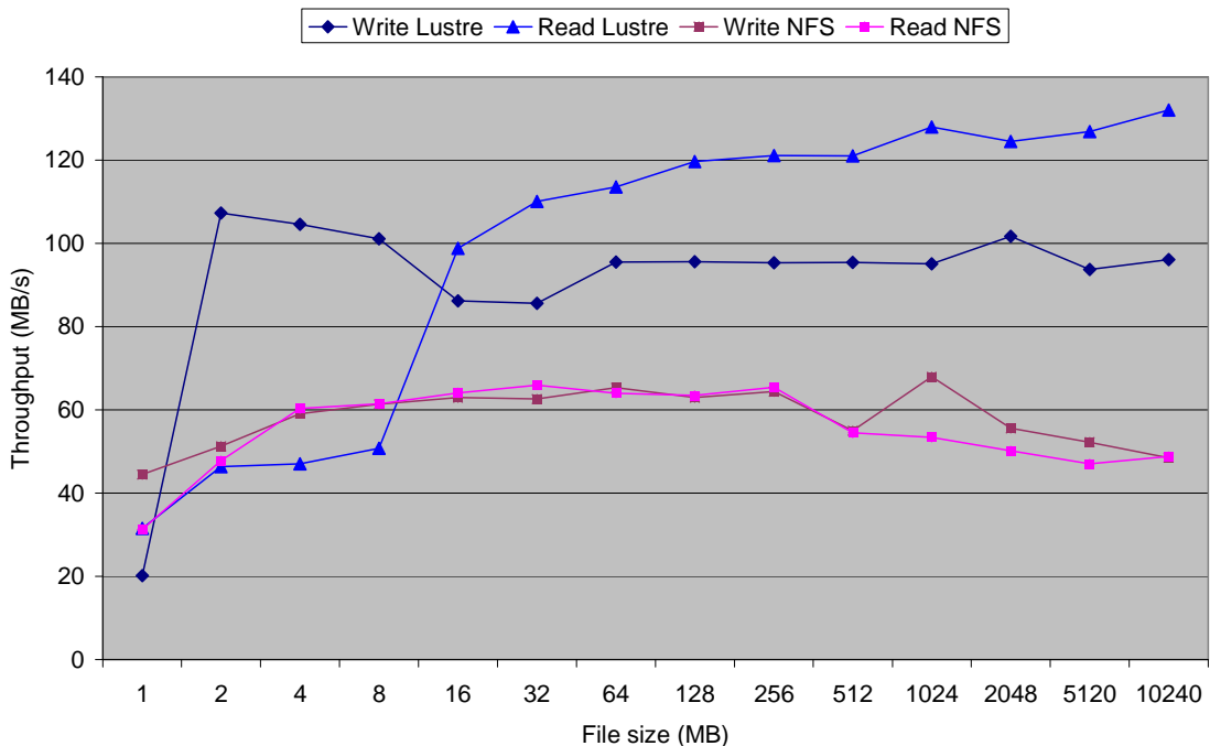
Figure 17 - Remote throughput depending on the file size
