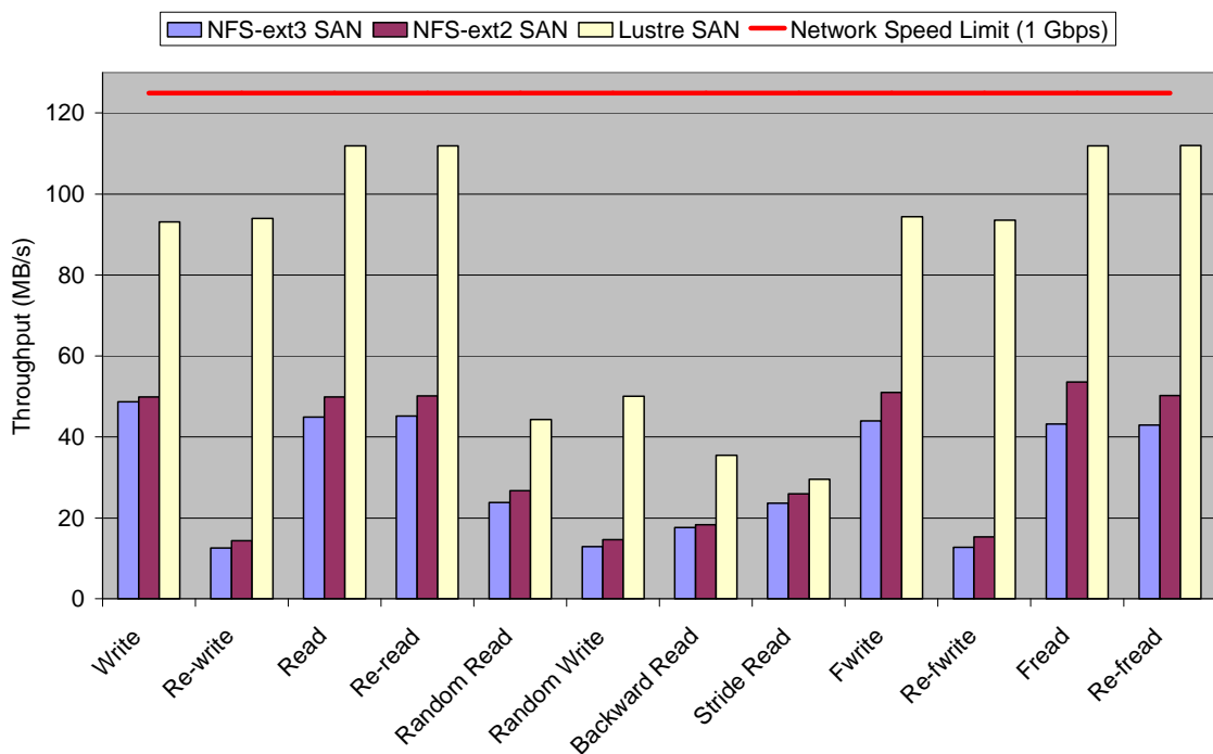
Figure 14 - Remote throughput
