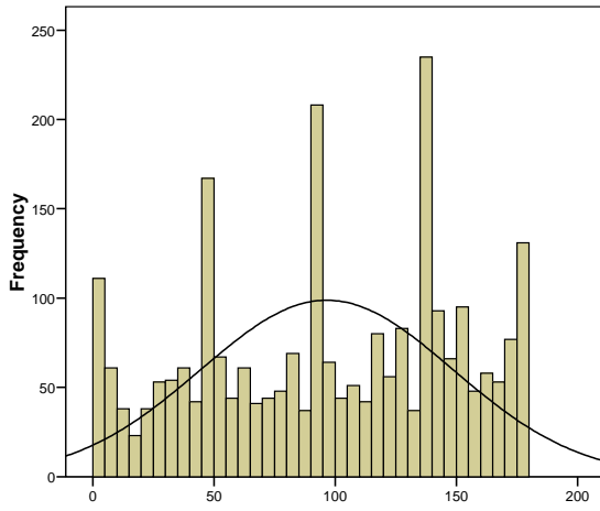
\alpha' – ASPECT [0-180] Unfailed
