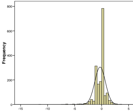
PL – PLAN CURVATURE Unfailed
