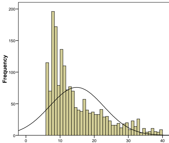
\beta - SLOPE Unfailed
