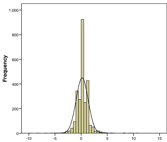
PF – PROFILE CURVATURE Unfailed
