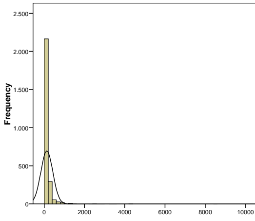
PENDM – MEAN WATERSHED SLOPE Unfailed
