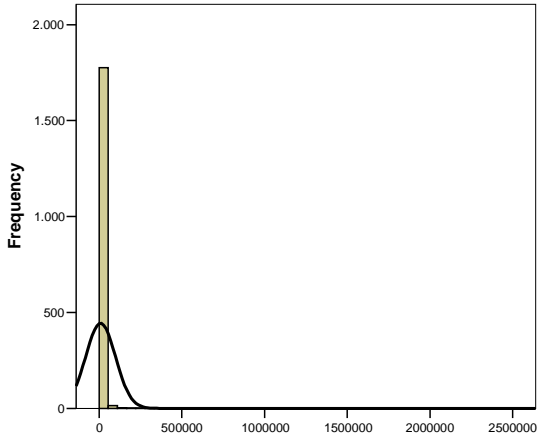
A – WATERSHED AREA Unfailed
