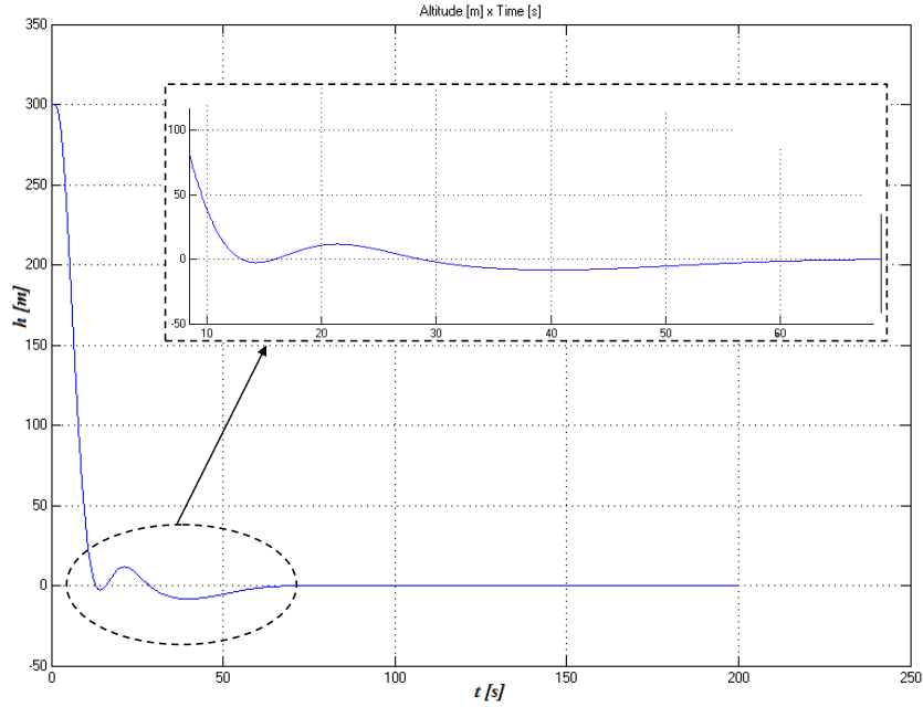
Fig. 6.1. Altitude Variation of Boeing 747-100 under flight conditions of case 1.1
