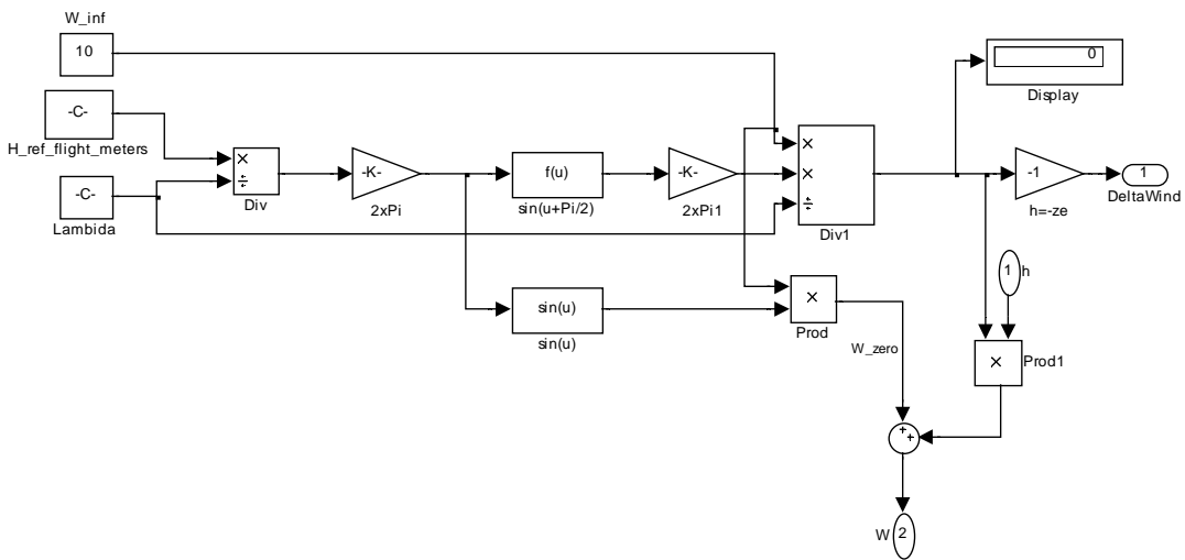
Fig. 5.21. Schema of WinData Subsystem for Exponential Wind Speed Profile
