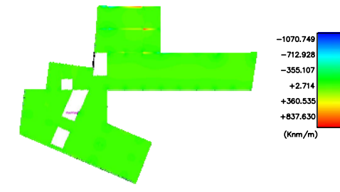
MOMENTS FLECTORS
