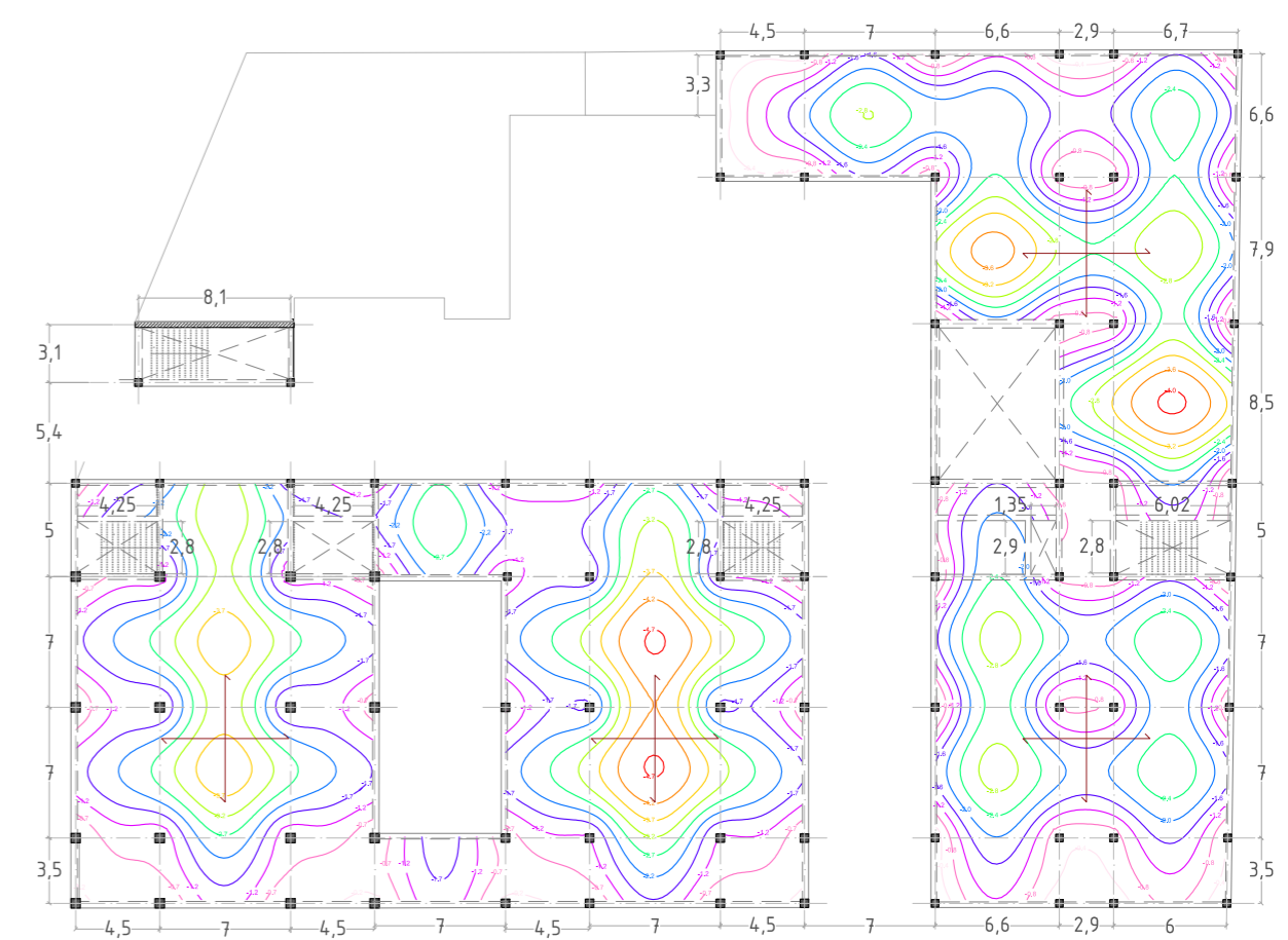
Isolinies sostre pb e. 1/400
