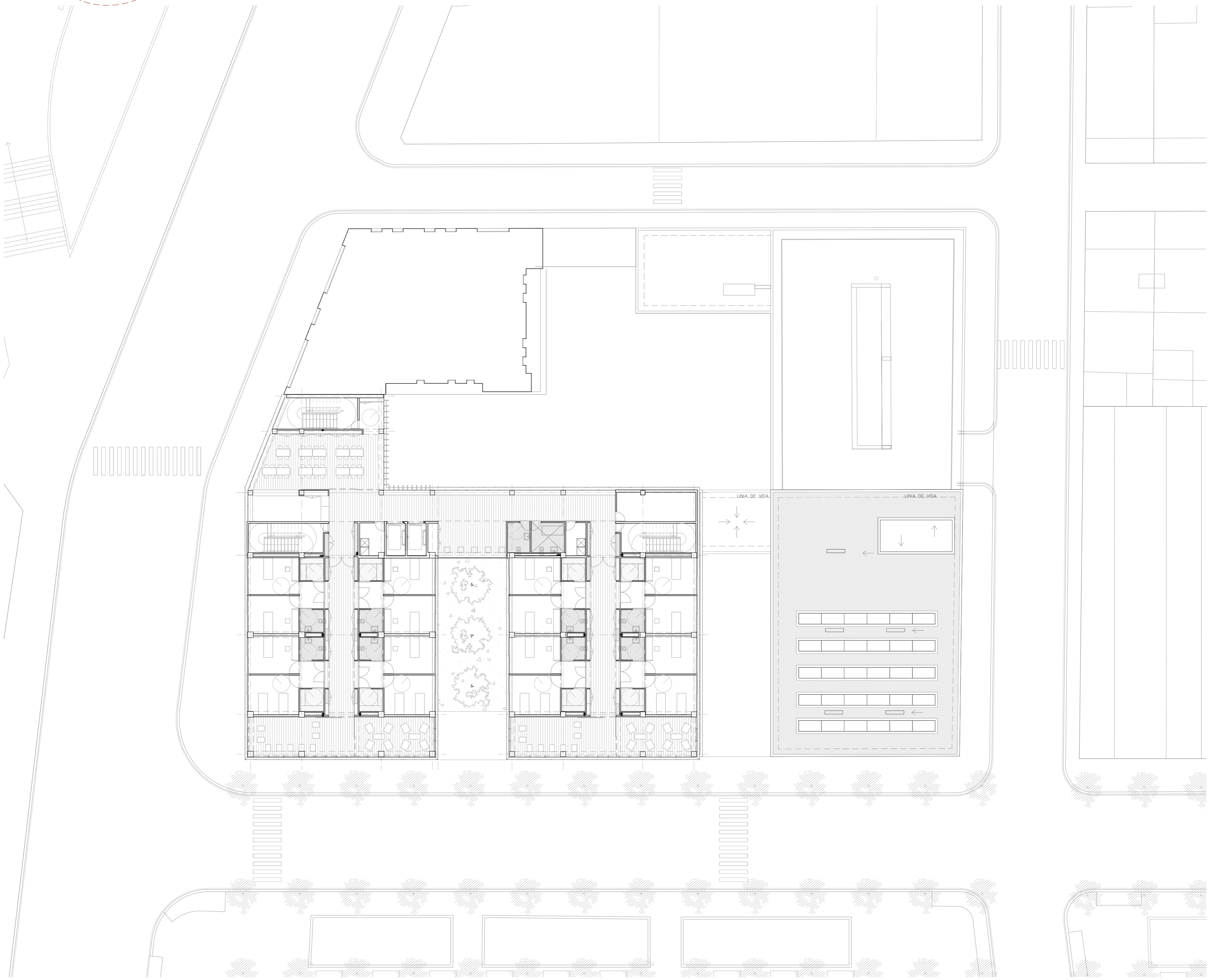
Planta pb+3 ( +10,08m)
