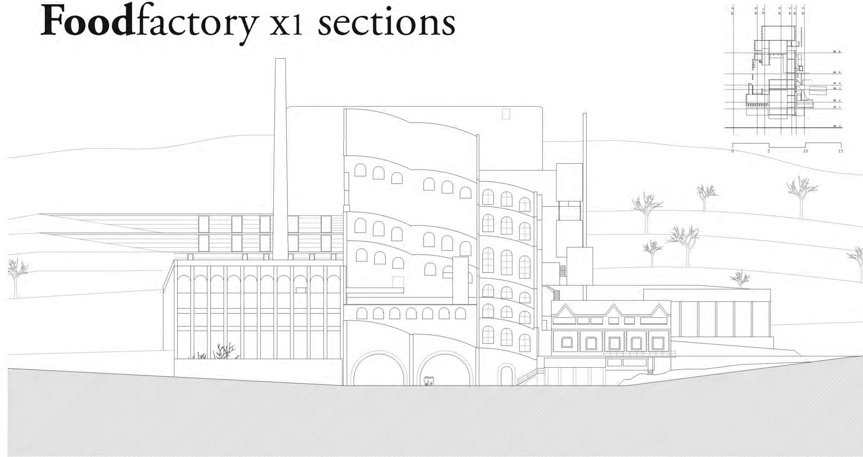
X0 South Elevation. 1.300
