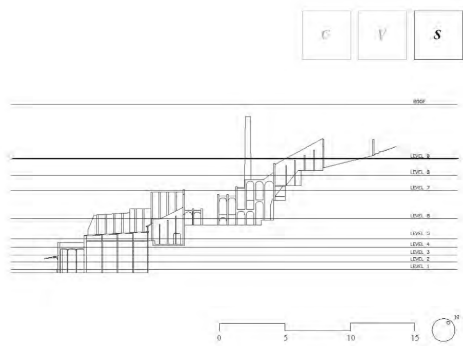
Level 9. Lodging access. 1.300
