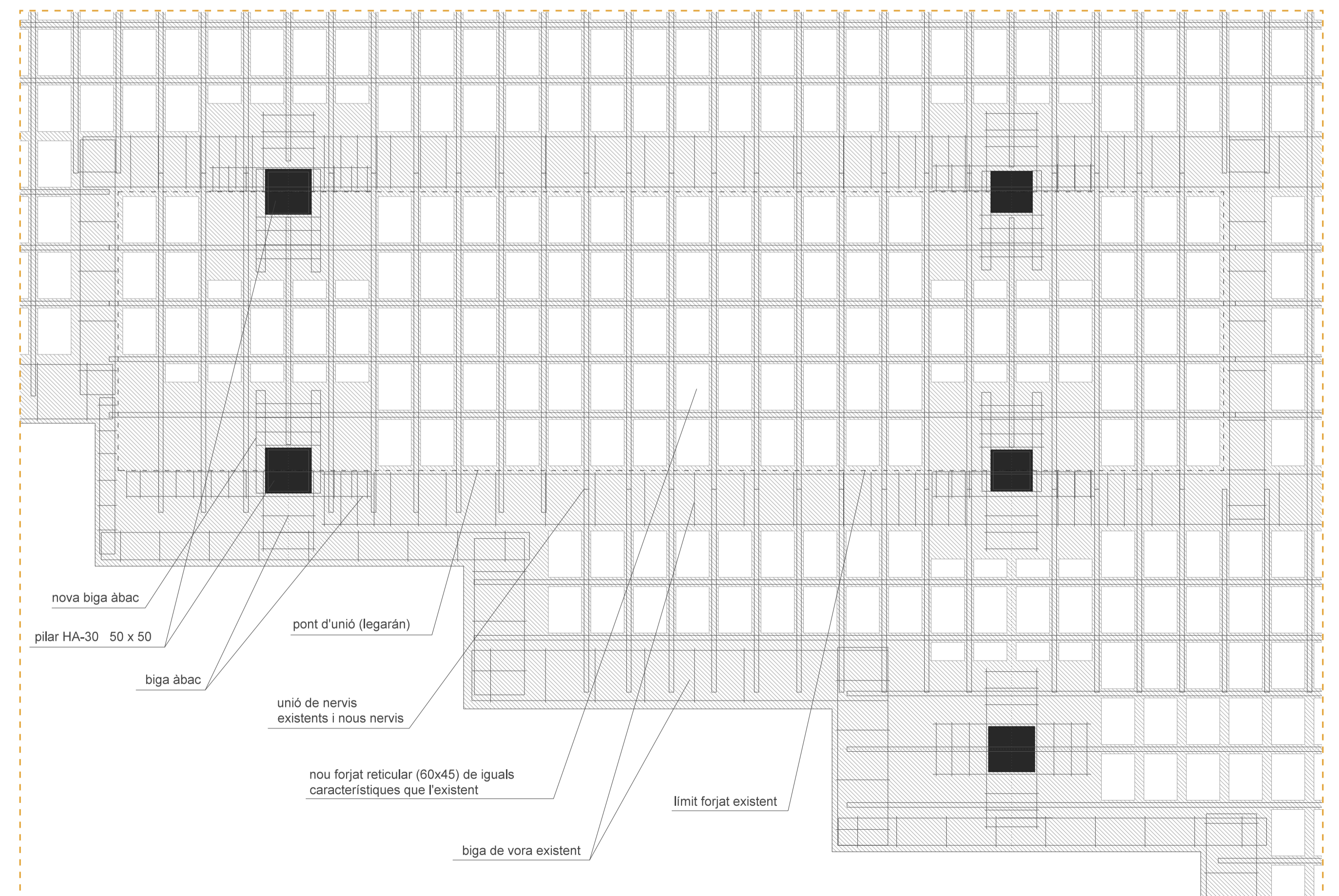
Detall 4 e: 1/40
