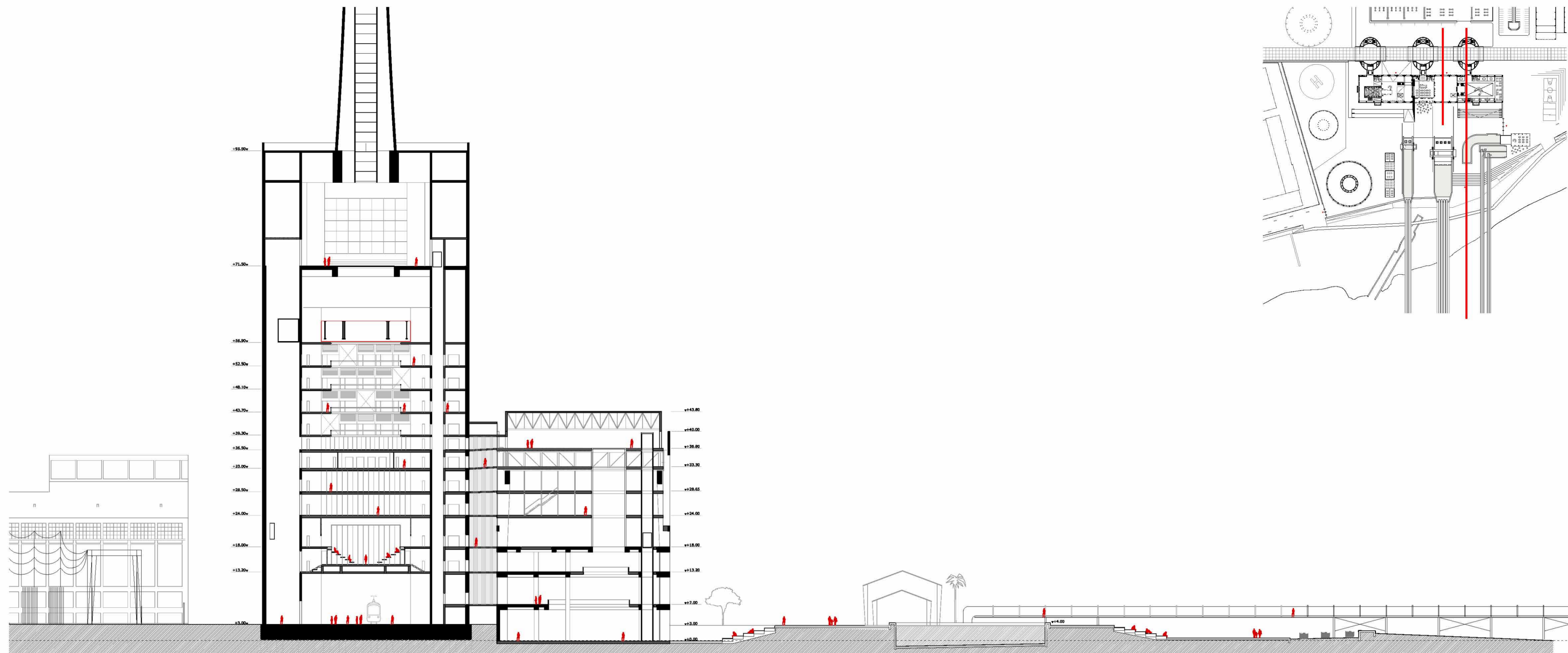
Section 14_15 E: 1|500
