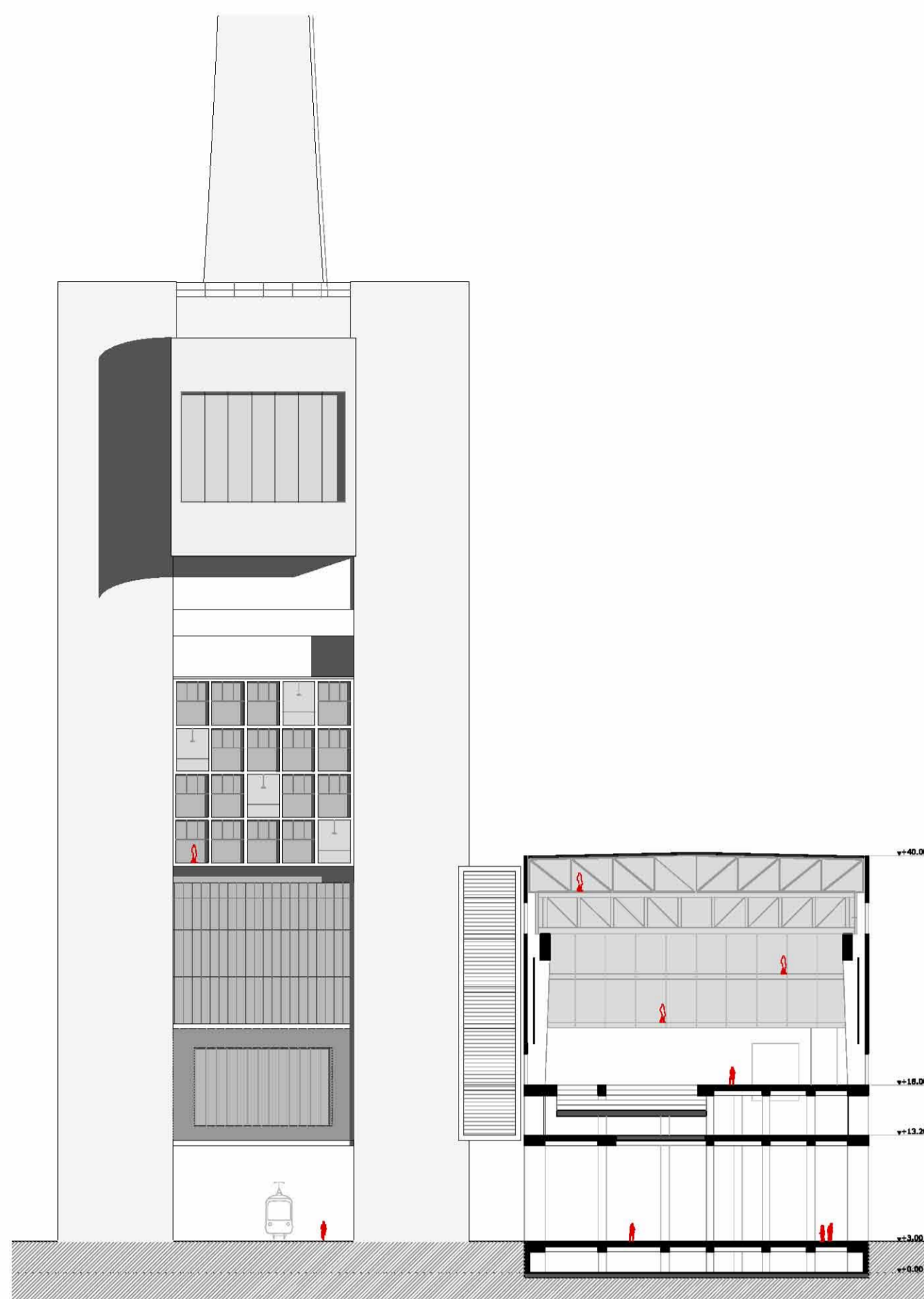
Section 11_12 E: 1|500
