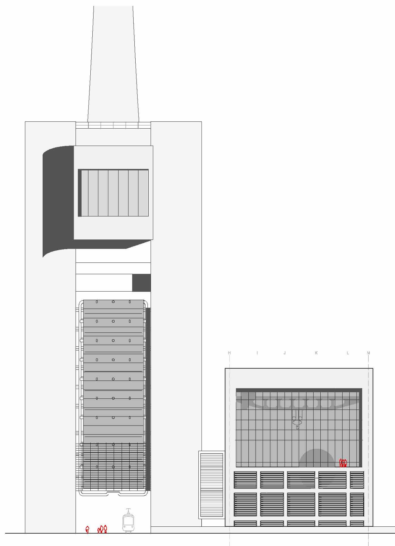
Elevation South-West E: 1/500
