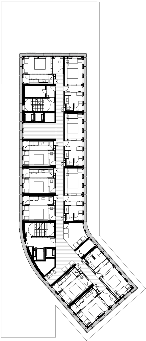
PLANTA TIPUS - HABITACIONS 8 PLANTES (+12.30m/+15.60/+18.90/+22.20/+25.50/+28.80/+32.10/+35.40)
