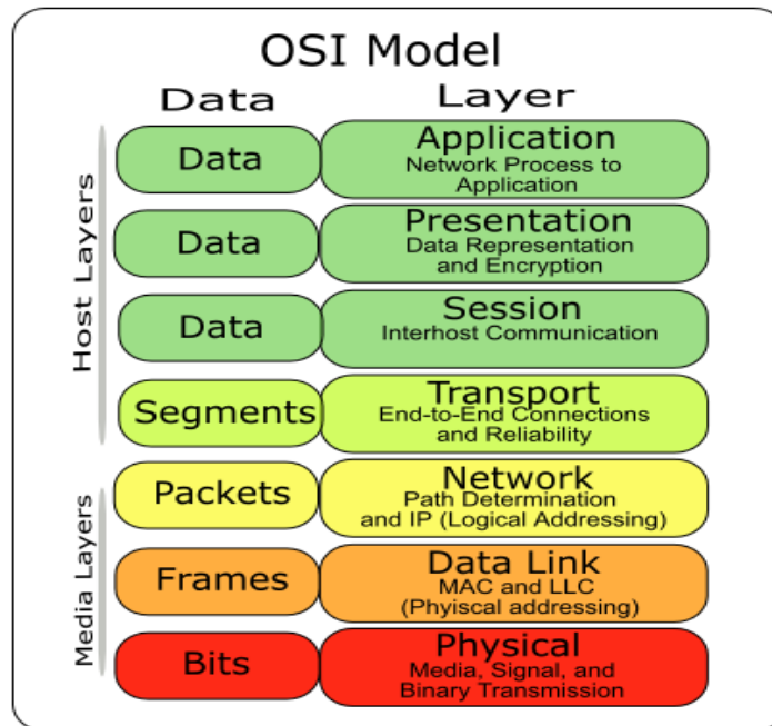
Fig 3.7 OSI model
