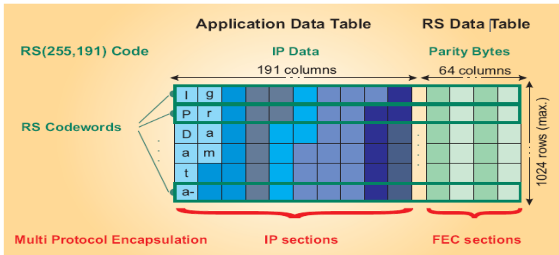
Fig. 4.3 MPE-FEC structure
