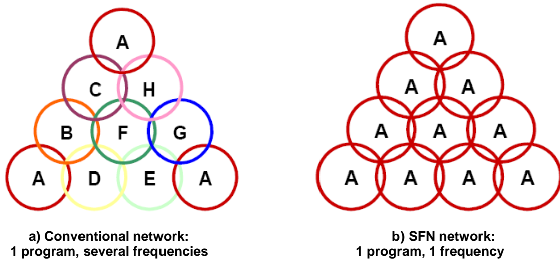
Fig. 3.8 Radiowaves planning
