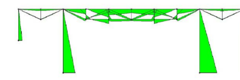
Moments
