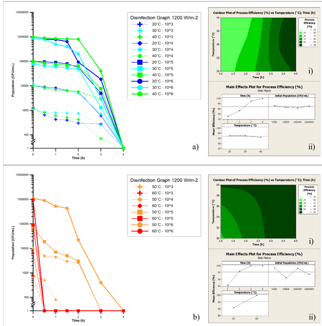
Figure 6 – Main results of 1200 W/m 2 experiments for synthetic secondary effluent at different temperatures and initial E. coli populations. (a) 20-40 °C Disinfection kinetic curves, a-i) 20-40 °C contour plot of process efficiency vs. temperature and time, a-ii) 20-40 °C Main effects plot (control variable: Process Efficiency). (b) 50-60 °C Disinfection kinetic curves, b-i) 50-60 °C contour plot of process efficiency vs. temperature and time, b-ii) 50-60 °C Main effects plot (control variable: Process Efficiency).
