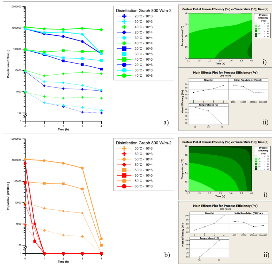
Figure 4 – Main results of 800 W/m 2 experiments for synthetic secondary effluent at different temperatures and initial E. coli populations. (a) 20-40 °C Disinfection kinetic curves, a-i) 20-40 °C contour plot of process efficiency vs. temperature and time, a-ii) 20-40 °C Main effects plot (control variable: Process Efficiency). (b) 50-60 °C Disinfection kinetic curves, b-i) 50-60 °C contour plot of process efficiency vs. temperature and time, b-ii) 50-60 °C Main effects plot (control variable: Process Efficiency).
