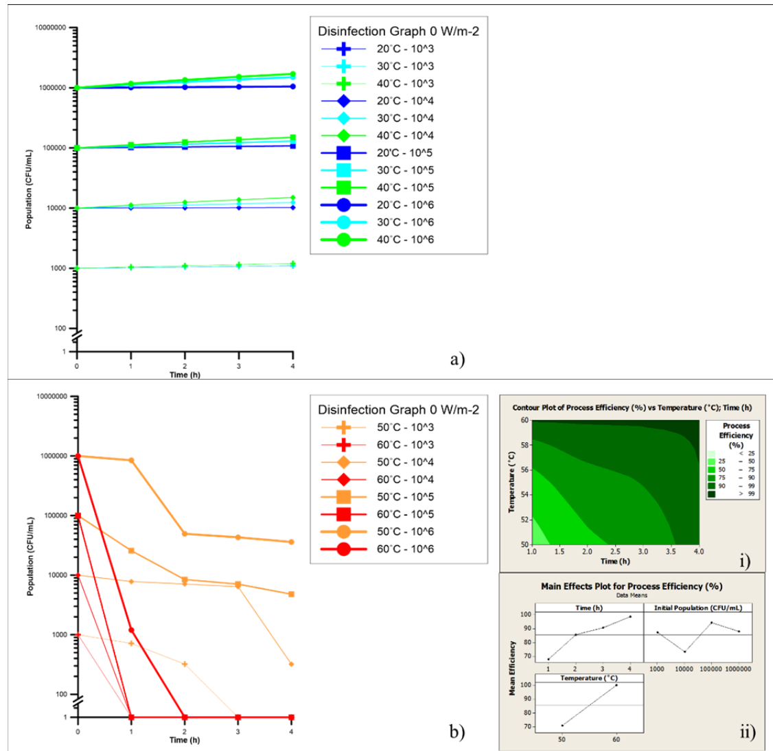
Figure 2 – Main results of non-irradiation experiments for synthetic secondary effluent at different temperatures and initial E. coli populations. (a) 20-40 °C kinetic curves. (b) 50-60 °C kinetic curves. b-i) Contour plot of the changes in process efficiency vs. temperature and time from 50-60 °C. b-ii) Main effects plot for temperatures 50-60 °C (control variable: Process Efficiency)
