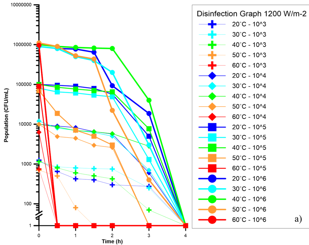
Figure 5 – Main results of 1200 W/m 2 experiments for synthetic secondary effluent at different temperatures and initial E. coli populations. (a) Disinfection kinetic curves. (b) Contour plot of process efficiency vs. temperature and time. (c) Main effects plot (control variable: Process Efficiency)
