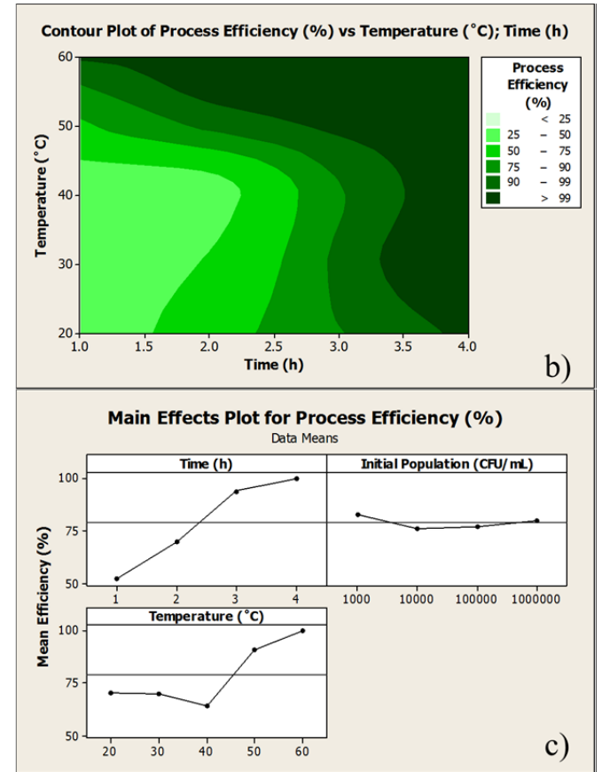
Figure 5 – Main results of 1200 W/m 2 experiments for synthetic secondary effluent at different temperatures and initial E. coli populations. (a) Disinfection kinetic curves. (b) Contour plot of process efficiency vs. temperature and time. (c) Main effects plot (control variable: Process Efficiency)
