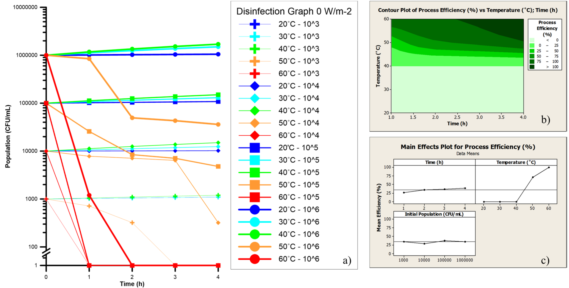
Figure 1 – Main results of non-irradiation experiments for synthetic secondary effluent at different temperatures and initial E. coli populations. (a) Disinfection kinetic curves. (b) Contour plot of process efficiency vs. temperature and time. (c) Main effects plot (control variable: Process Efficiency)
