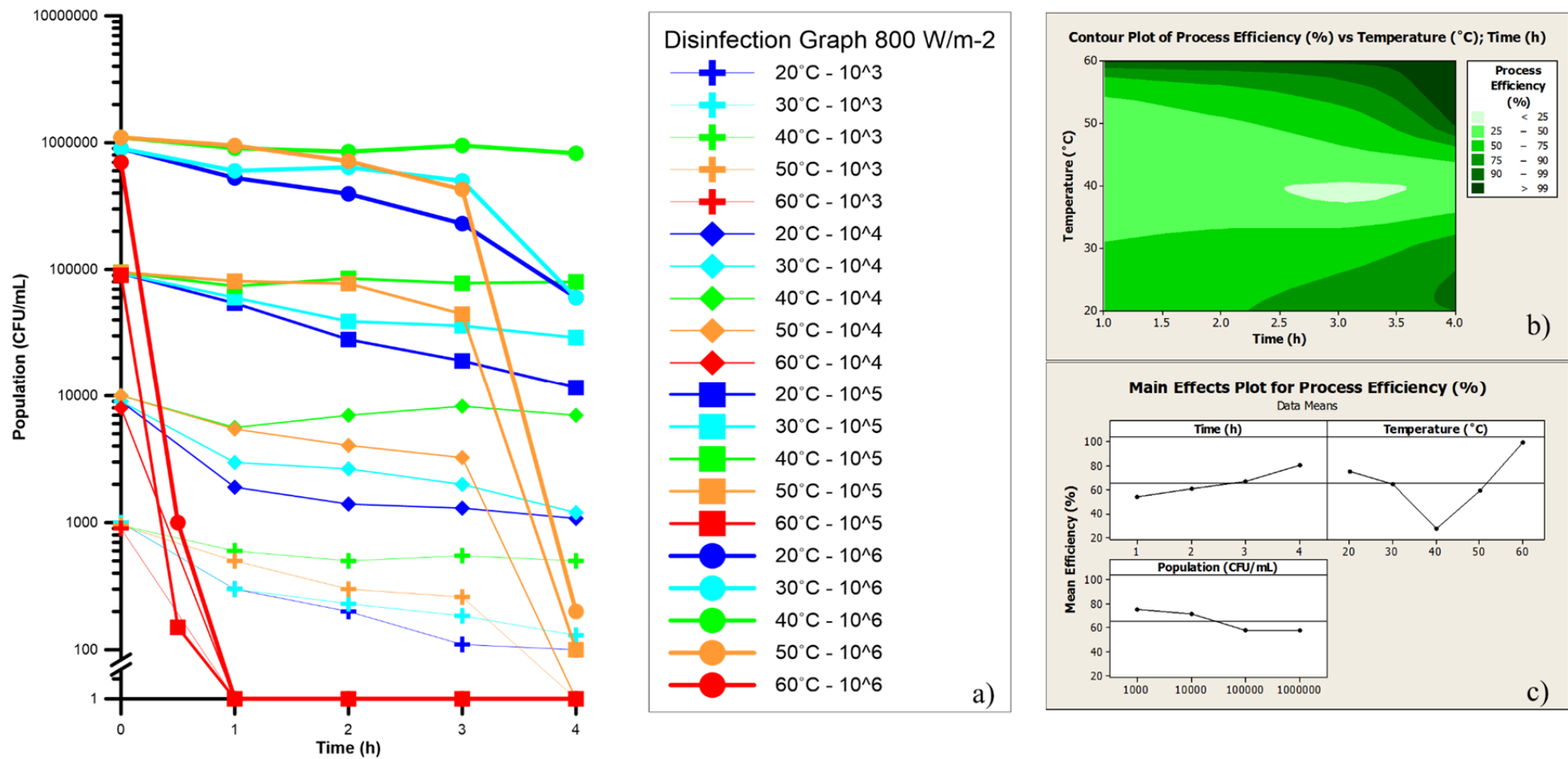
Figure 3 – Main results of 800 W/m 2 experiments for synthetic secondary effluent at different temperatures and initial E. coli populations. (a) Disinfection kinetic curves. (b) Contour plot of process efficiency vs. temperature and time. (c) Main effects plot (control variable: Process Efficiency)
