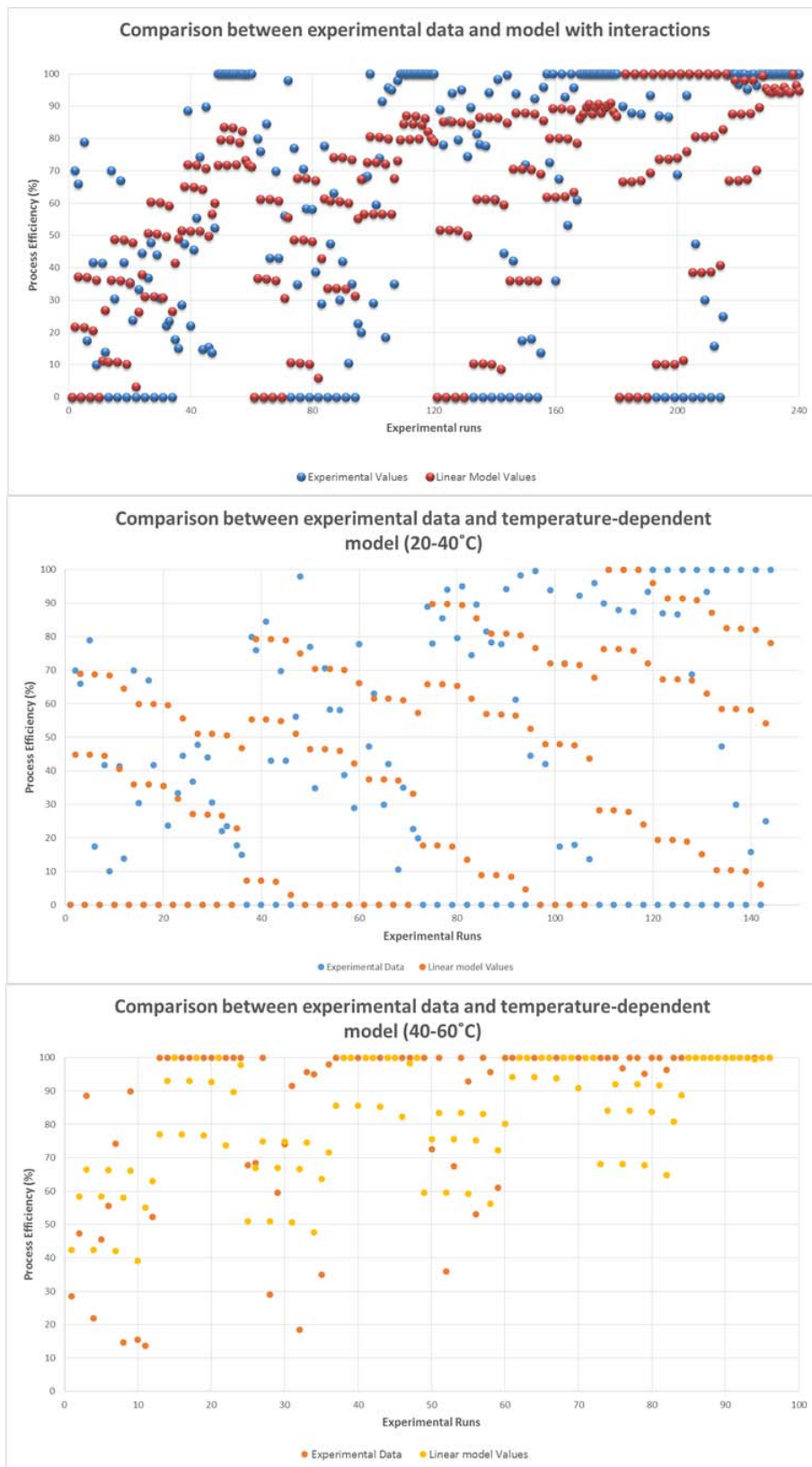
Figure 7 – Fitting of the linear models to the experimental data. (a) Linear model with interactions. (b) Temperature dependent model (20-40°C). (c) Temperature dependent model (40-60°C).
