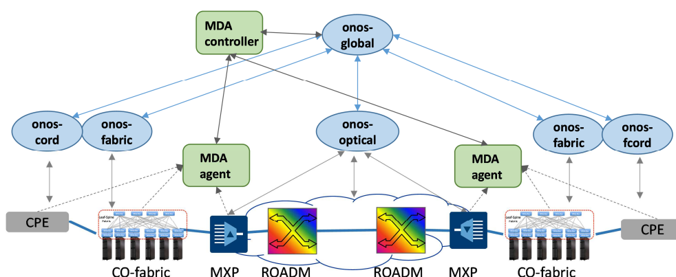
Fig. 1: Network controllers view and monitoring architecture
