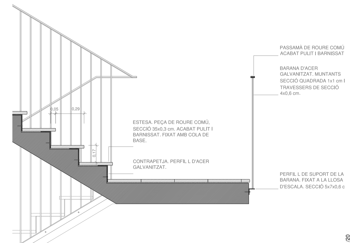
DETALLS_MATERIALS ACABAT 1/20
