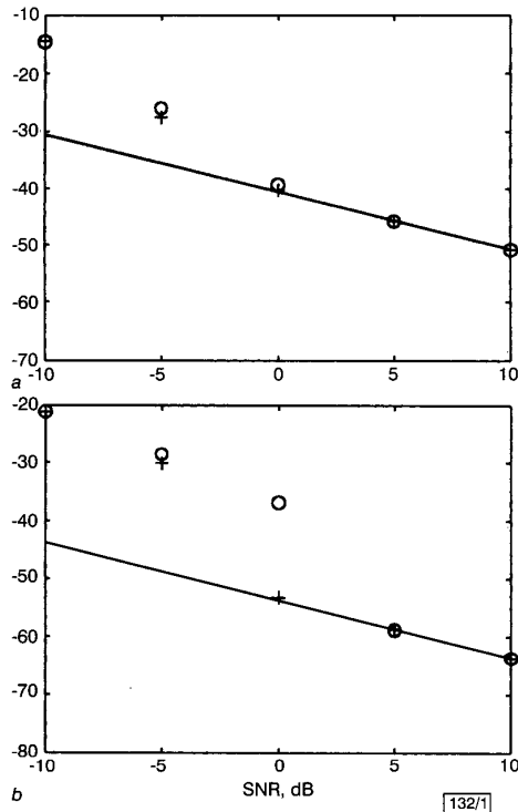
Fig. 1 Comparison of MSEs obtained via DS-WRELAX and FML algorithms with corresponding CRBs for \tau_1 and \sigma_1
