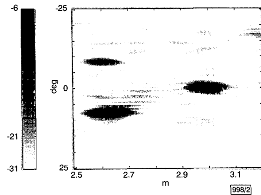
Fig. 2 Quick-CSAR reflectivity image (two trihedrals and one sphere)
