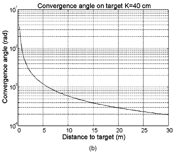
Fig. 3 (a) Diameter 2w_0 of the transmitted-beam waist as a function of distance d_3 to target on which it is assumed to lie, and (b) convergence angle of transmitted beam 2q_0 as a function of distance d_3 to the target on which the beam waist is assumed to lie.
