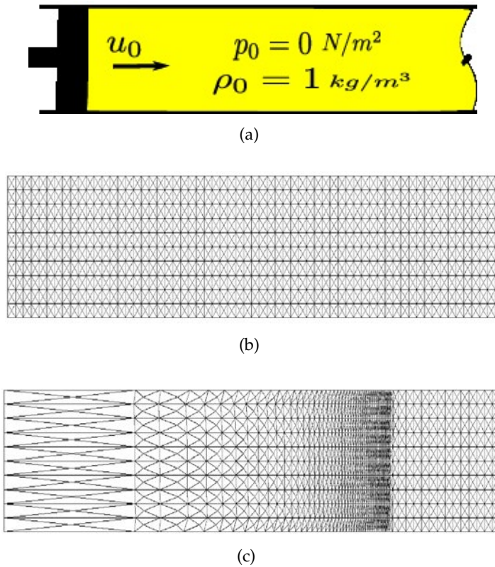
Figure 3.12: 1D Sedov test. a) constant initial density, b) initial mesh configuration, c) mesh configuration for t = 1.0s
