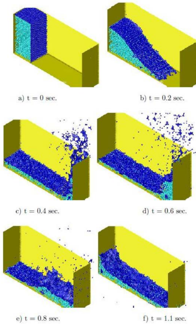
Figure 2.6: 3D dambreak modelled in the PFEM [92].
