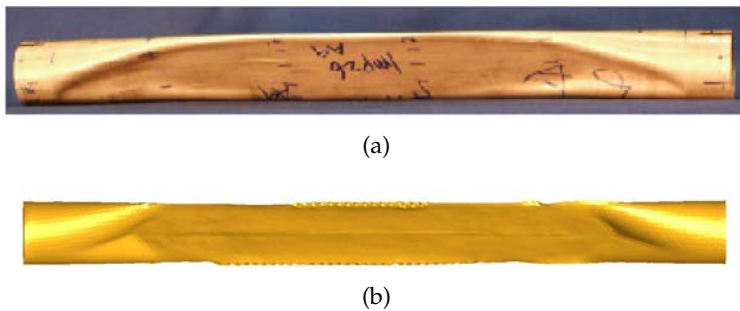
Figure 5.8: Final configuration of cylinder a) experiment, b) simulation
