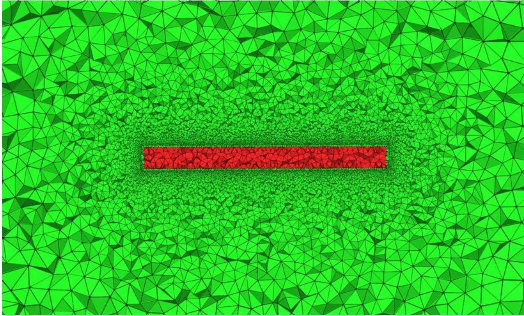
Figure 5.7: Mesh configuration inside and near the cylinder at the beginning of the simulation.
