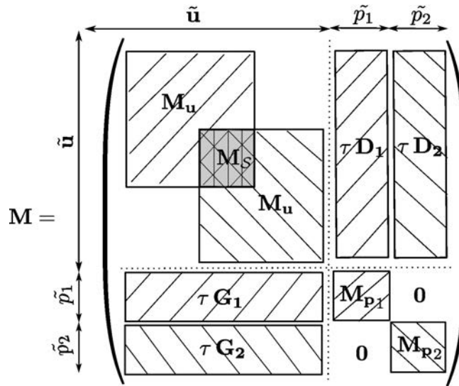
Figure 5.4: Coupled mass matrix. M_s represents the contribution of the shell element to the coupled system. Note that each domain has its own pressure variables that are duplicated at the interface nodes (Figure 5.3).
