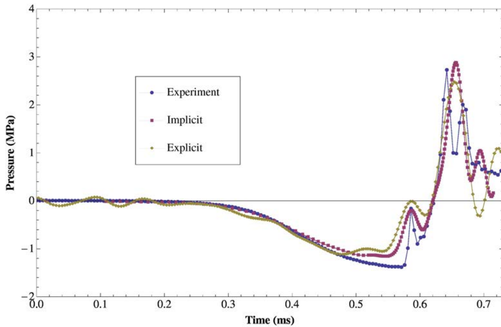
Figure 5.9: Time history of pressure in one of the sensors compared with implicit and explicit results. Zero pressure corresponds to the initial pressure of 6.99 MPa.
