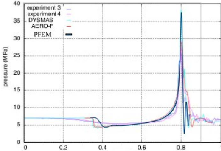
Figure 3.25: Time history of pressure at 10.16 cm from the center of the bubble
