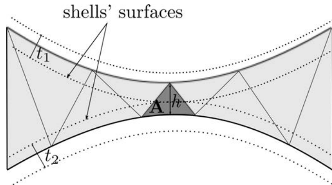
Figure 5.2: Shell thicknesses t_1 and t_2 and actual distance between mid-planes, h . Light gray zone is the potential contact domain discretized by triangular elements. Element “A” in dark gray is an active element that satisfies the contact criteria.
