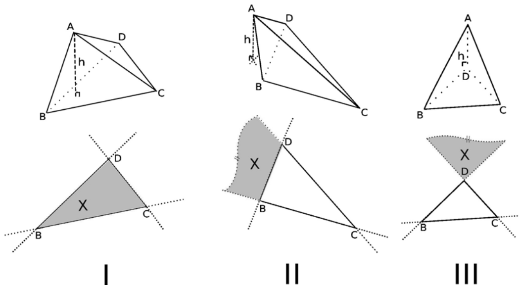
Figure 4.4: Vertex-edge combinations
