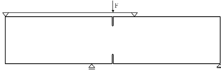
Figure 7.12: Double notched four points beam: schematical diagram of the applied loads in the experimental test.
