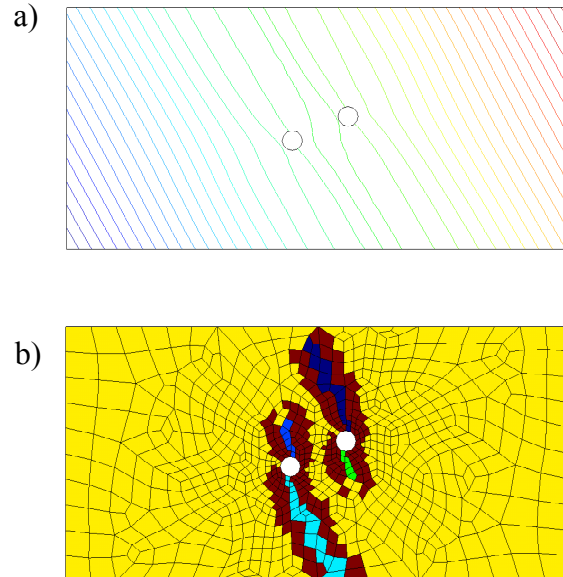
Figure 7.19: Plate with two geometrical imperfections: a) discontinuity lines, b) exclusion zone (elements in dark brown).
