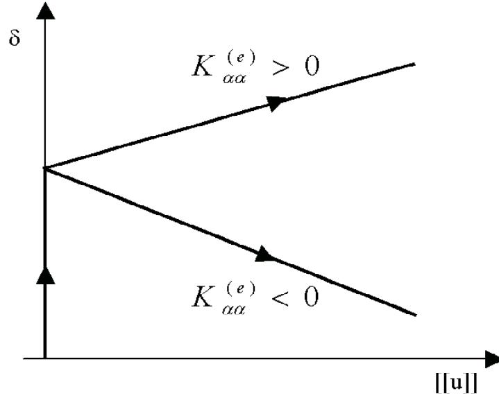
Figure 6.2: Nodal displacement vs. elemental jump in a one dimensional element.
