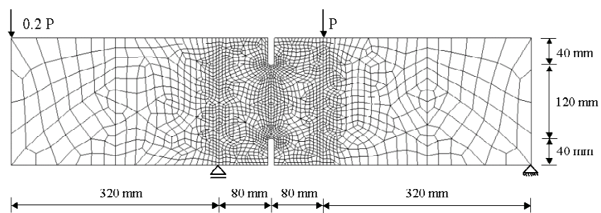
Figure 7.11: Double notched four points bending test: mesh and boundary conditions.
