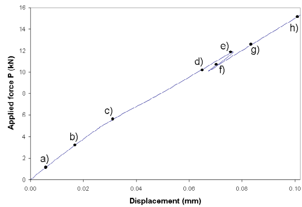
Figure 7.36: Tension pull specimen (fine mesh): global response curve indicating the loading levels at which pictures of the cracking state will be taken.
