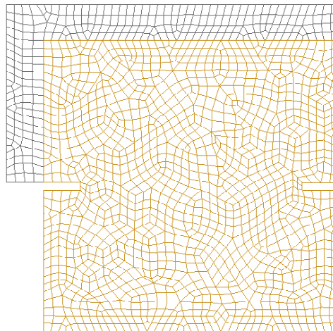
Figure 7.24: Mixed mode test: mesh.
