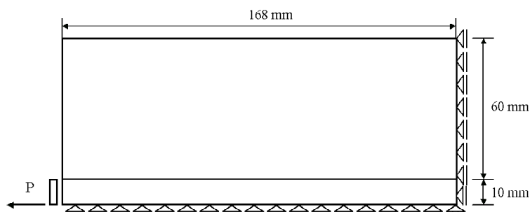
Figure 7.29: Tension pull specimen: geometry.
