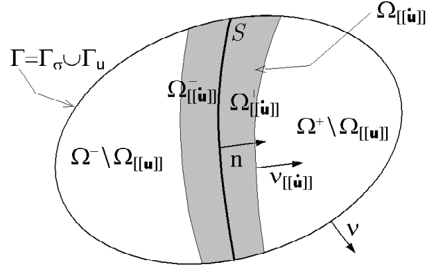
Figure B.1: Solid with a strong discontinuity.
