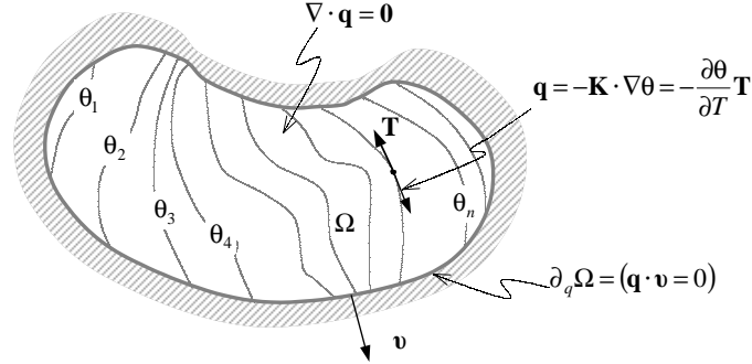
Figure 5.5: Heat-conduction-like boundary value problem.
