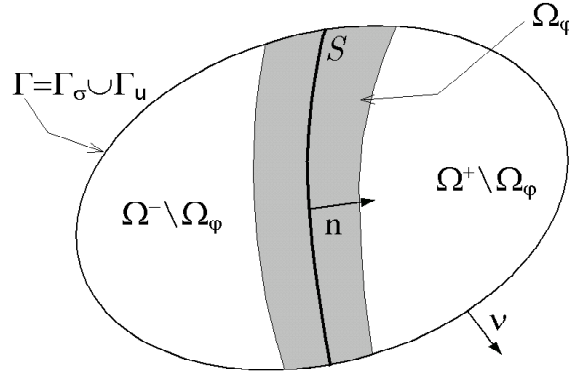
Figure 4.1: Solid with a strong discontinuity interface.
