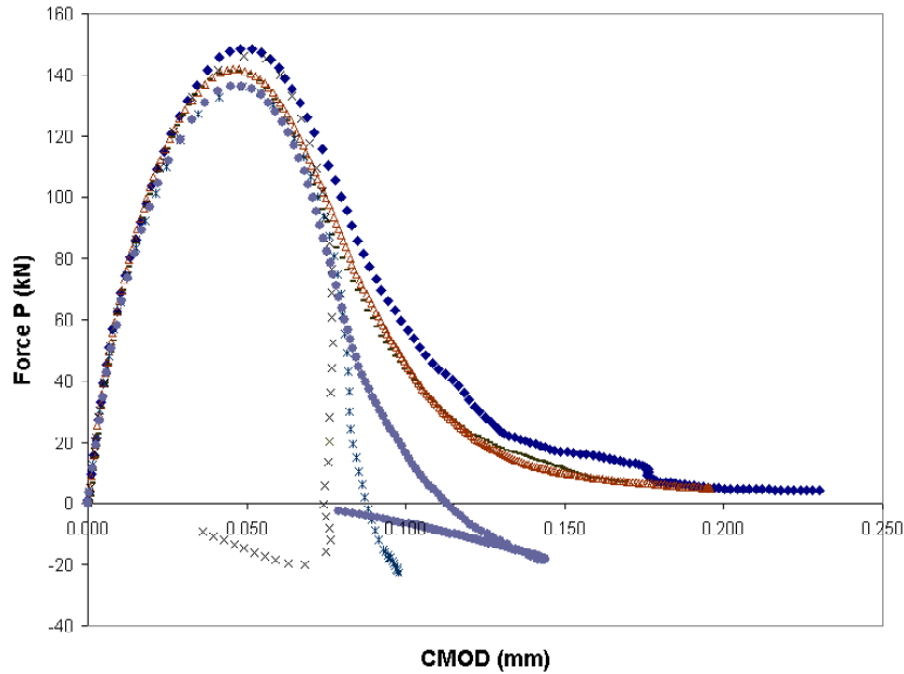
Figure 7.4: Single notched four points bending test: comparison of the global response of several meshes.
