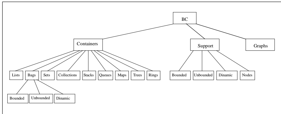
Figure 1: Hierarchy of the Booch component classes (excerpt).
