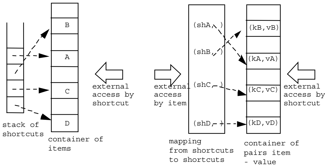
Figure 5: Adding shortcuts to linear structures (left) and to mappings (right).
