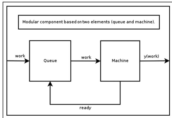
Figure 6. Coupled Discrete Event System Specification model combining two models, one representing a Queue and the other a Machine.
