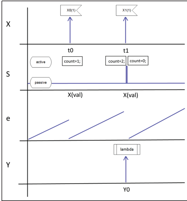
Figure 15. Trajectories for the binary counter model showing the Specification and Description Language (SDL) elements that will be represented on the equivalent SDL model. The states can be “passive” and “active”; when an external event is received (represented by the INPUT element), the variable “count” is increased by the value. In S we can see that the internal event is triggered when \text{count} > 2 . Also, Y represents the PROCEDURE that implements the lambda Discrete Event System Specification function.
